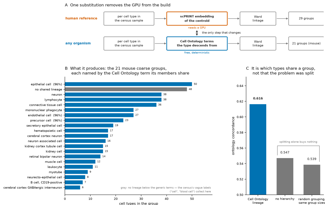
Figure 4. Replacing the one step of the reference build that needs a GPU. A : both routes to the coarse groups; only the middle step differs. B : the 21 coarse groups of broad_mouse_v1 , each named by the Cell Ontology term its members share, with a percentage where that term covers most but not all of the group; the gray bar is the single group whose members share no term below the generic ones. C : the ontology grouping against no hierarchy and against a random grouping with the same group sizes, scored by ontology concordance on the held-out human lung atlas.
