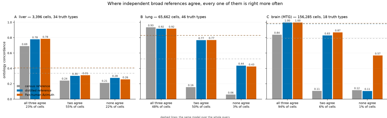
Figure 2. Ontology concordance within each agreement tier for three broad references, on withheld cross-study liver (A), the Krasnow lung atlas (B) and the Allen human middle temporal gyrus (C); dashed lines are the same models over the whole query. Agreement is evaluated in the Cell Ontology because the three references answer in different vocabularies (798, 382 and 324 classes). The ordering is the same in all three tissues; the fraction of cells on which the references agree is not, and tracks how finely the query’s own annotation is resolved.
