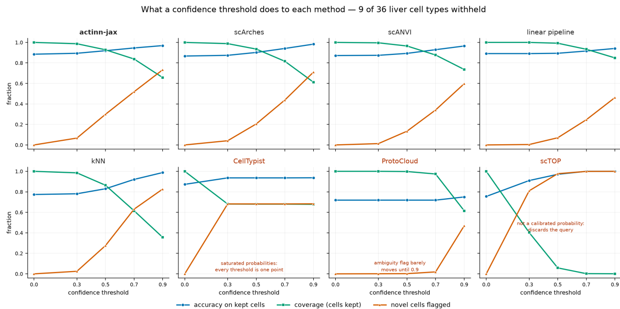
Figure S8. What a confidence threshold does to each of the eight methods that return a per-cell confidence, with 9 of 36 cell types held out of the liver reference so 1,350 query cells are out-of-distribution. Every quantity is a fraction, so all three share one axis. The five that work share a shape — accuracy and novelty rising as coverage falls — and the three that do not each fail visibly and differently.
