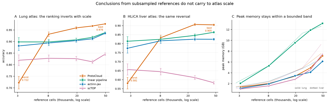
Figure S5. Accuracy and peak memory against reference size, four methods carried to full atlas scale on two datasets. A : lung, 3k \rightarrow 49k reference cells. B : the HLiCA liver atlas, 2.7k \rightarrow 47k, an independent replication of the same reversal — a prototype VAE moves from worst to best as the reference grows. C : peak memory over both sweeps. Error bars on A and B are 95% binomial
