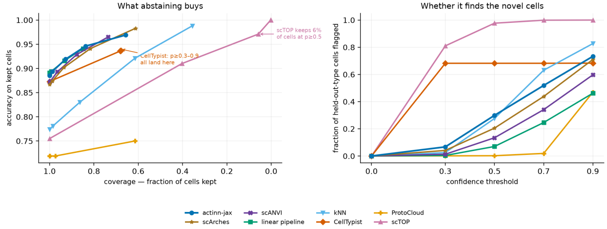
Figure S9. The same sweep read as a trade-off, which is what compares methods to each other rather than to themselves. Left: accuracy on kept cells against the fraction kept — the five usable methods lie along one band, which is the basis for calling their abstain quality tied. Right: the share of held-out-type cells flagged as the threshold rises.
