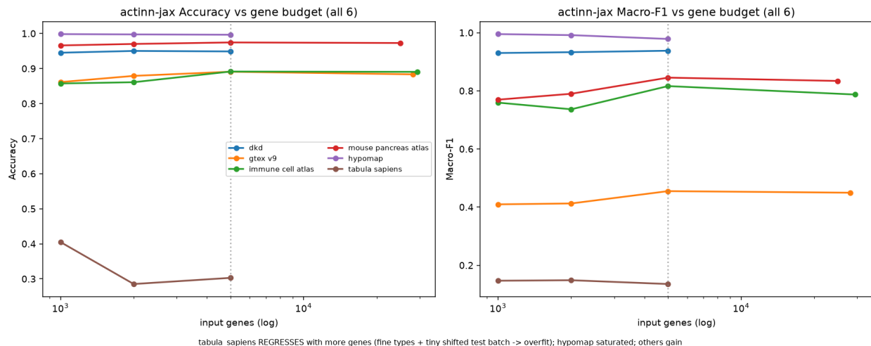
Figure 5. actinn-jax accuracy and macro-F1 against input gene budget across all six Open Problems datasets. More genes help most datasets but regress the fine-grained, domain-shifted tabula_sapiens.
