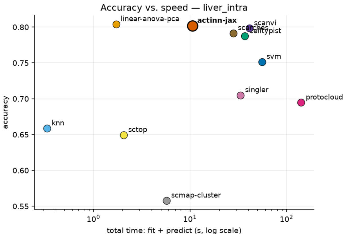
Figure 2. Accuracy against total wall time on liver_intra . The tuned linear pipeline holds the fast-frontier point; actinn-jax sits just inside it at this reference size, and what separates it is visible only on the scaling axes of Figure 3.
