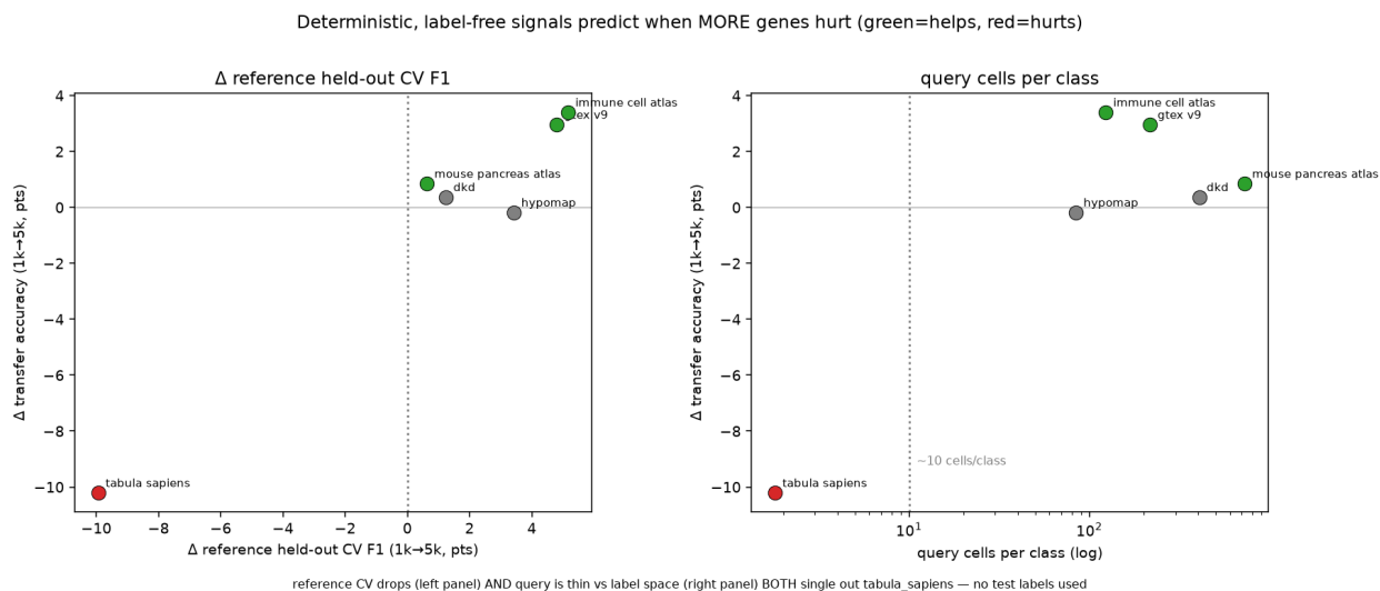
Figure 6. Label-free signals for setting the gene budget without test labels. Held-out reference cross-validation and query-cells-per-class both single out tabula_sapiens, the one dataset where more genes hurt.
