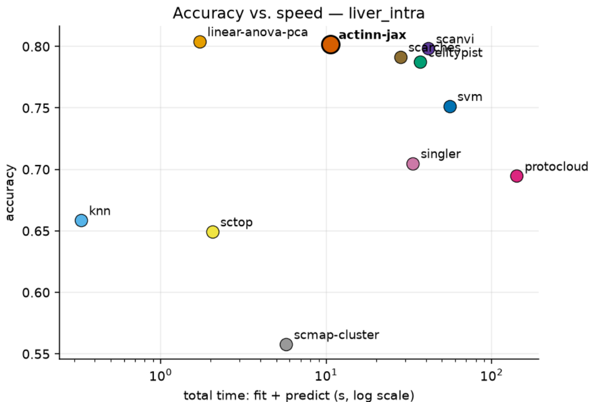
Figure 1. Accuracy against total wall time on liver_intra. The tuned linear pipeline holds the fast-frontier point; actinn-jax sits just inside it at this reference size, and what separates it is visible only on the scaling axes of Figure 2.
