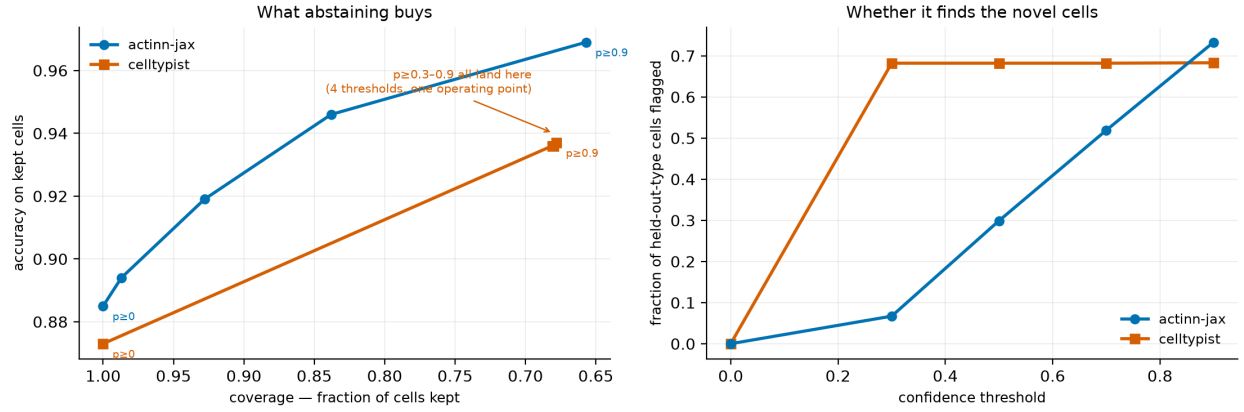
Figure S2. Abstention with 9 of 36 liver cell types withheld from the reference, so 1,350 query cells are genuinely out of distribution. Left: accuracy on kept cells against coverage. Right: the fraction of held-out-type cells flagged as the threshold rises. actinn-jax traces a usable curve on both axes; CellTypist’s probabilities are saturated, so thresholds from 0.3 to 0.9 land on a single operating point and its novel-cell detection is flat from 0.3 onward.
