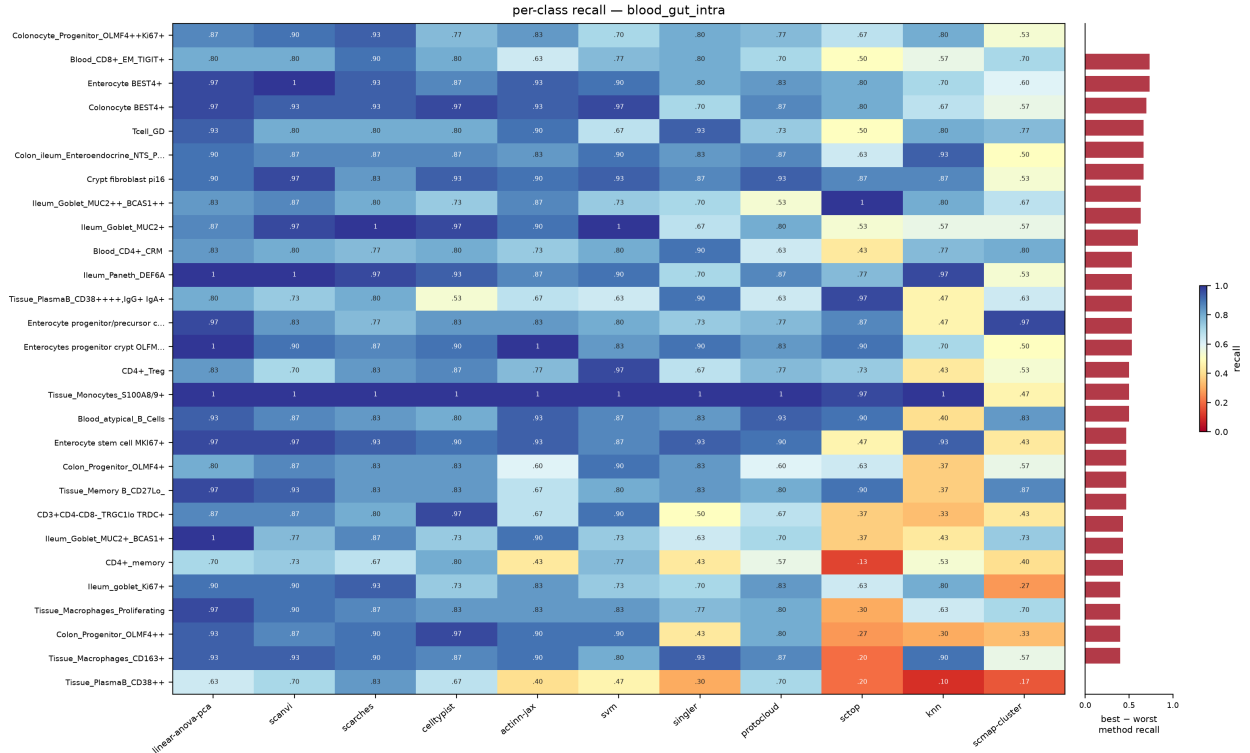
Figure S3. Per-class recall for eleven methods on the 86-type blood+gut split, ordered by how much the methods disagree (best minus worst recall, right-hand strip). The best and worst method differ by a median of 0.30 recall per class and up to 0.73; mean pairwise Spearman between methods’
