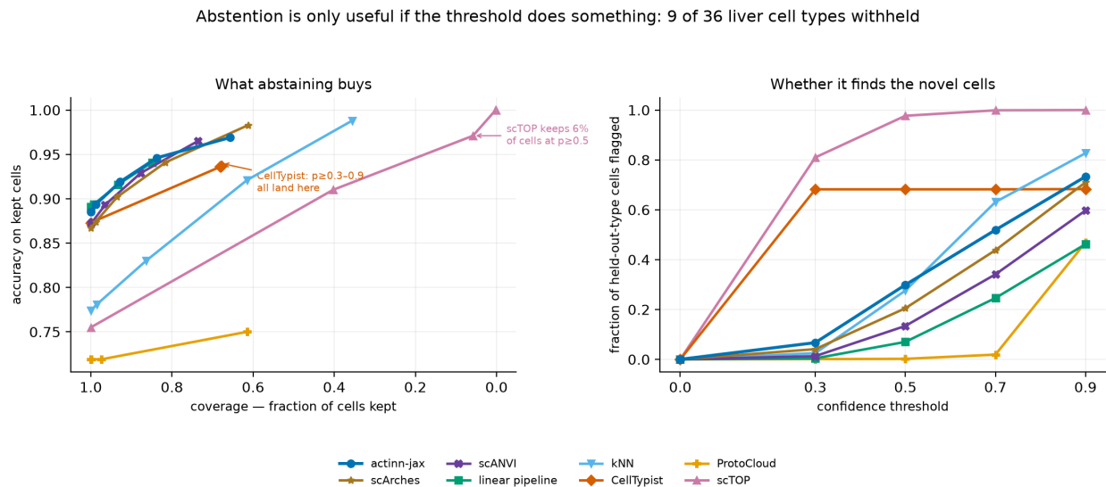
Figure 8. The same sweep read as a trade-off, which is what compares methods to each other rather than to themselves. Left : accuracy on kept cells against the fraction kept — the five usable methods lie along one band, which is the basis for calling their abstain quality tied. Right : the share of held-out-type cells flagged as the threshold rises. The three methods Figure 7 shows failing appear here as curves that go nowhere along one axis or the other.
