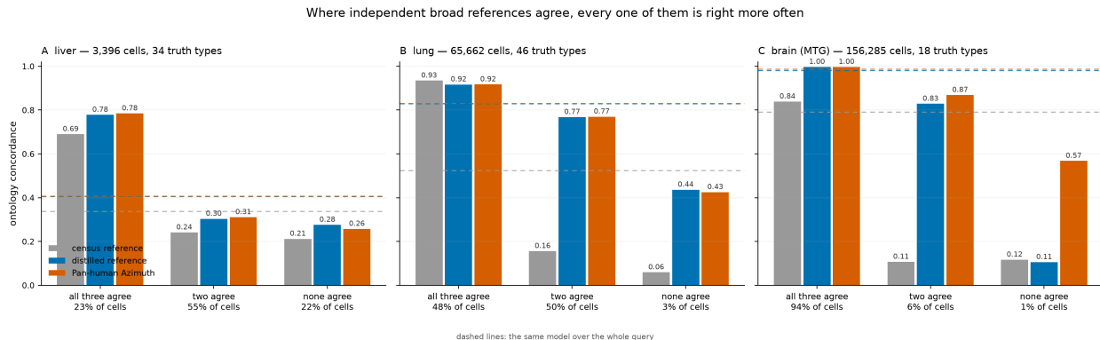
Figure 3. Ontology concordance within each agreement tier for three broad references, on withheld cross-study liver ( A ), the Krasnow lung atlas ( B ) and the Allen human middle temporal gyrus ( C ); dashed lines are the same models over the whole query. Agreement is evaluated in the Cell Ontology because the three references answer in different vocabularies (798, 382 and 324 classes). The ordering is the same in all three tissues; the fraction of cells on which the references agree is not, and tracks how finely the query’s own annotation is resolved.
