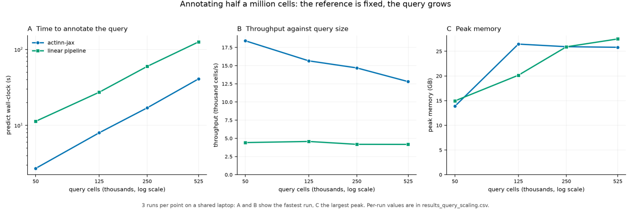
Figure 4. Cost against query size with the reference fixed at 17,753 cells. A : wall-clock to annotate the query. B : throughput, which declines 31% for actinn-jax and holds flat for the linear pipeline, narrowing the advantage from 4.2 \times to 3.1 \times . C : peak memory, which does not distinguish them – on this axis it measures holding the query, not running the method. Three runs per point on a shared laptop: A and B report the fastest run, since contention can only add time, and C the largest peak, since resident-set size understates a run that the OS has partly evicted. Per-run values are in results_query_scaling.csv .
