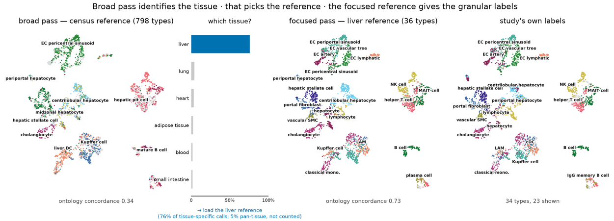
Figure 5. The workflow on a withheld HLiCA liver study (3,396 cells), same embedding throughout. Left : the shipped census reference spreads 144 of its 798 labels over the query (concordance 0.34 ) — it is not trying to name subtypes. Center : those calls resolved to tissue through the reference’s per-class tissue map; 76% of tissue-specific calls say liver against 4% for the next candidate, which is the decision that selects the next reference. Right of center : the 36-type liver reference re-annotates the same cells at 0.73 , now tracking the clusters. Right : the study’s own labels on the shared palette. Both models are leakage-free for this query: the focused reference is trained only
