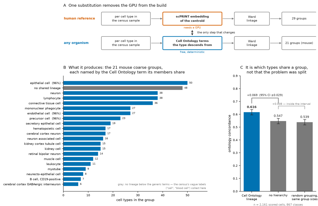
Figure 6. Replacing the one step of the reference build that needs a GPU. A : both routes to
