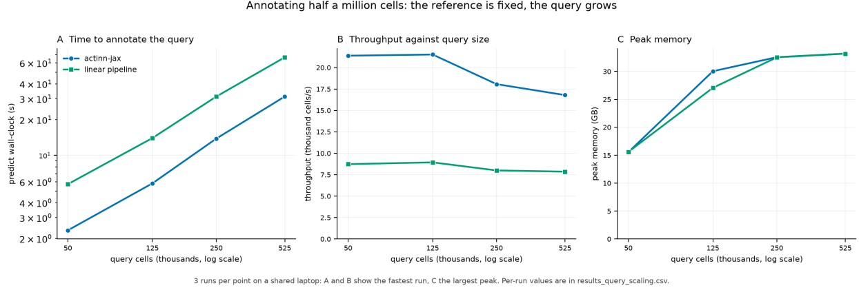
Figure 4. Cost against query size — 50,000 to 524,699 cells — with the reference fixed at 17,753 cells. Table 3’s queries are all smaller than the leftmost point here (657 to 13,550 cells), so the two do not overlap. A : wall-clock to annotate the query. B : throughput, which declines 21% for actinn-jax and 10% for the linear pipeline, narrowing the advantage from 2.4× to 2.1×. C : peak memory, which does not distinguish them — on this axis it measures holding the query, not running the method. Three runs per point on a shared laptop: A and B report the fastest run, since contention can only add time, and C the largest peak, since resident-set size understates a run that the OS has partly evicted. Per-run values are in results_query_scaling.csv .
