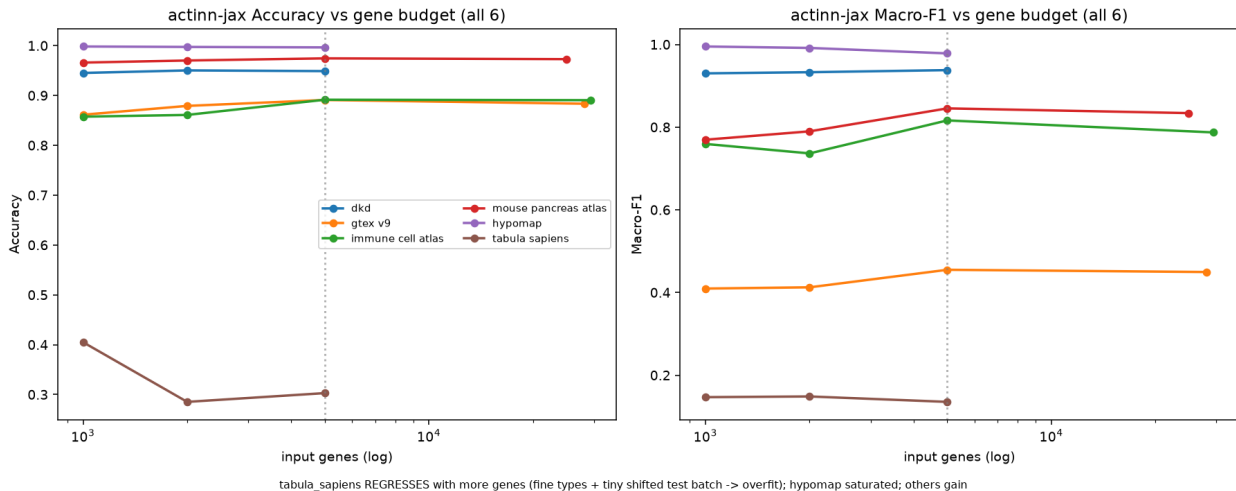
Figure 6. actinn-jax accuracy and macro-F1 against input gene budget across all six Open Problems datasets. More genes help most datasets but regress the fine-grained, domain-shifted tab-
