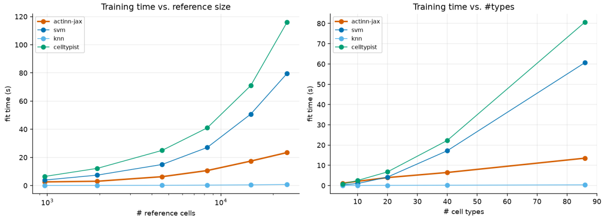
Figure 1. Fit and prediction time against reference size and label cardinality. Fit grows for every trained method; prediction stays flat and sub-second across the whole range.
