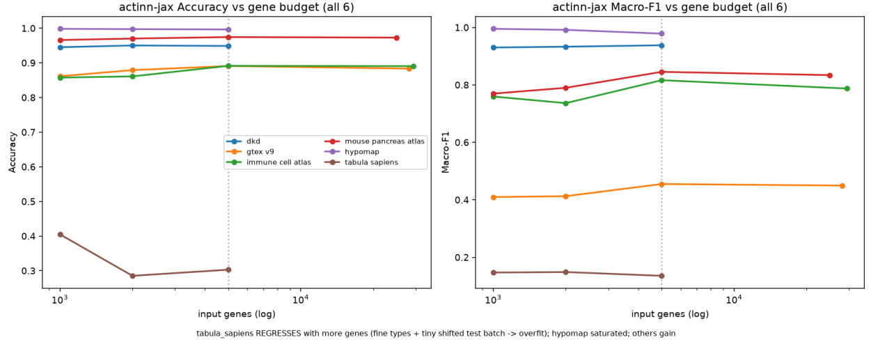
Figure S12. actinn-jax accuracy and macro-F1 against input gene budget across all six Open Problems datasets. More genes help most datasets but regress the fine-grained, domain-shifted tabula_sapiens .
