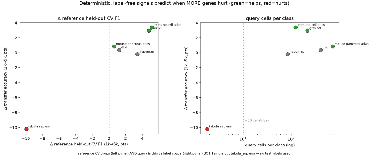
Figure S13. Label-free signals for setting the gene budget without test labels. Held-out reference cross-validation and query-cells-per-class both single out tabula_sapiens , the one dataset where more genes cost real accuracy — about 10 points. hypomap drifts down as well, but from a saturated 0.998, and neither signal flags it.
