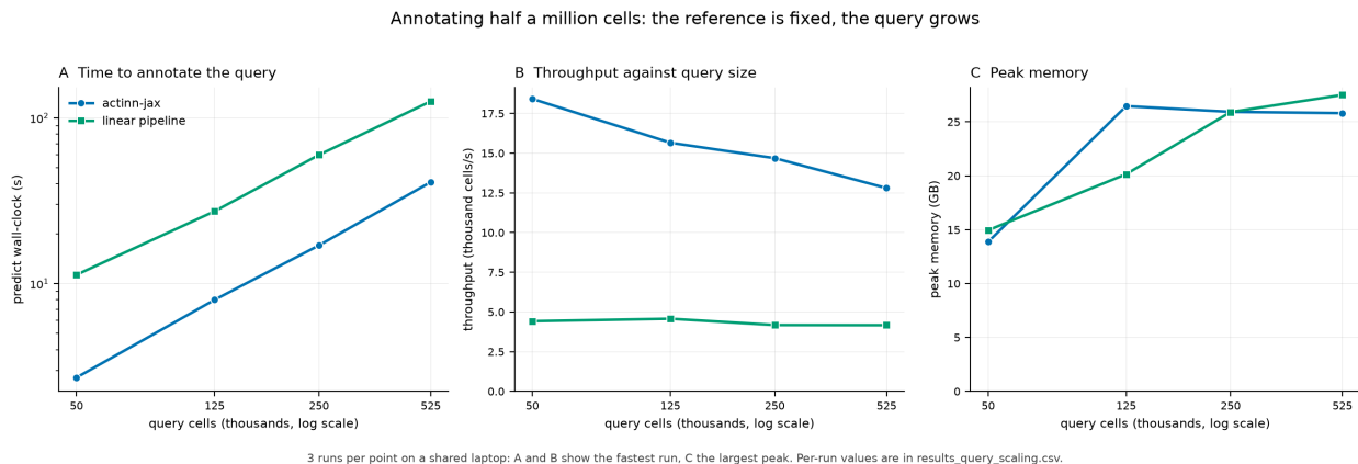
Figure S8. Cost against query size — 50,000 to 524,699 cells — with the reference fixed at 17,753 cells; every query in the main accuracy panel is smaller than the leftmost point here. A : wall-clock to annotate the query. B : throughput, which declines 31% for actinn-jax and holds flat for the linear pipeline, narrowing the advantage from 4.2 \times to 3.1 \times . C : peak memory, which does not distinguish them — on this axis it measures holding the query, not running the method. Three runs per point on a shared laptop: A and B report the fastest run, since contention can only add time, and C the largest peak, since resident-set size understates a run the OS has partly evicted.
