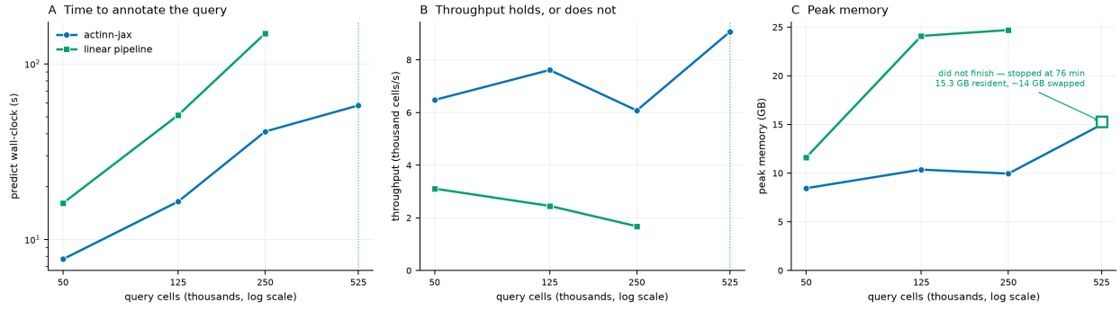
Figure 4. Cost against query size with the reference fixed at 17,753 cells. A : wall-clock to annotate the query. B : throughput, which holds for actinn-jax and falls for the linear pipeline. C : peak memory; the open marker is the linear pipeline’s unfinished 524,699-cell run, drawn at the memory still resident when it was stopped and deliberately not joined to its curve, since the rest of its working set had been evicted to swap. Wall-clock is a single run on a laptop and carries scheduling noise, which is why B is not monotone for either method.
