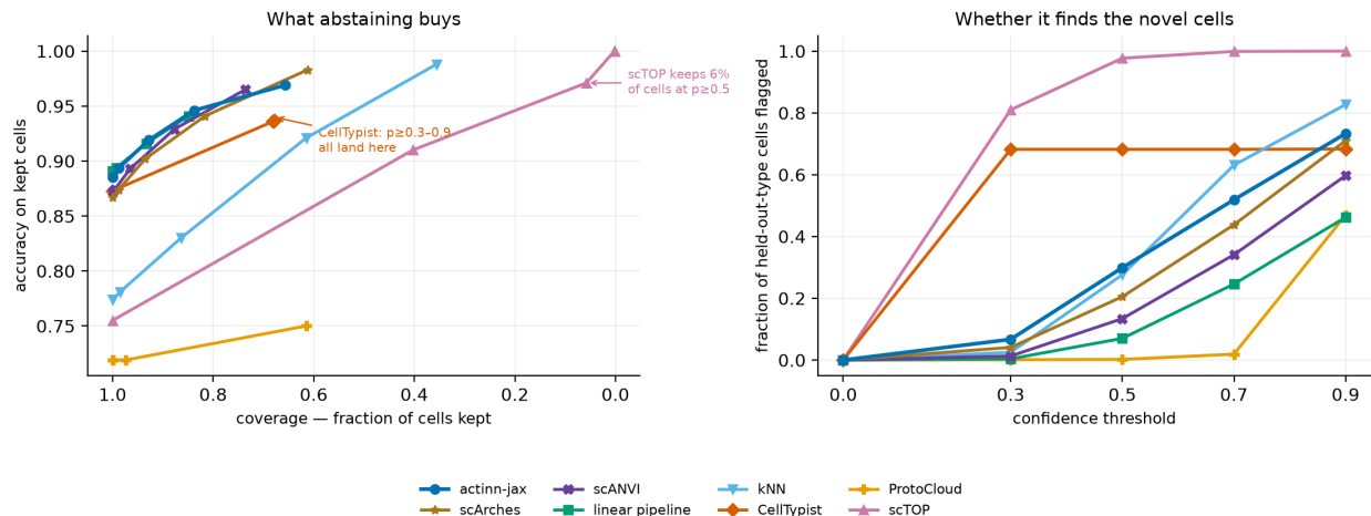
Figure 7. What abstention buys, and whether it finds the novel cells, for the eight methods that return a per-cell confidence. Left: accuracy on kept cells against the fraction kept. Right: the share of held-out-type cells flagged as the threshold rises. A usable mechanism moves along both axes; CellTypist’s saturated probabilities collapse four thresholds onto one operating point, and scTOP’s projection score discards the query rather than ranking it.
