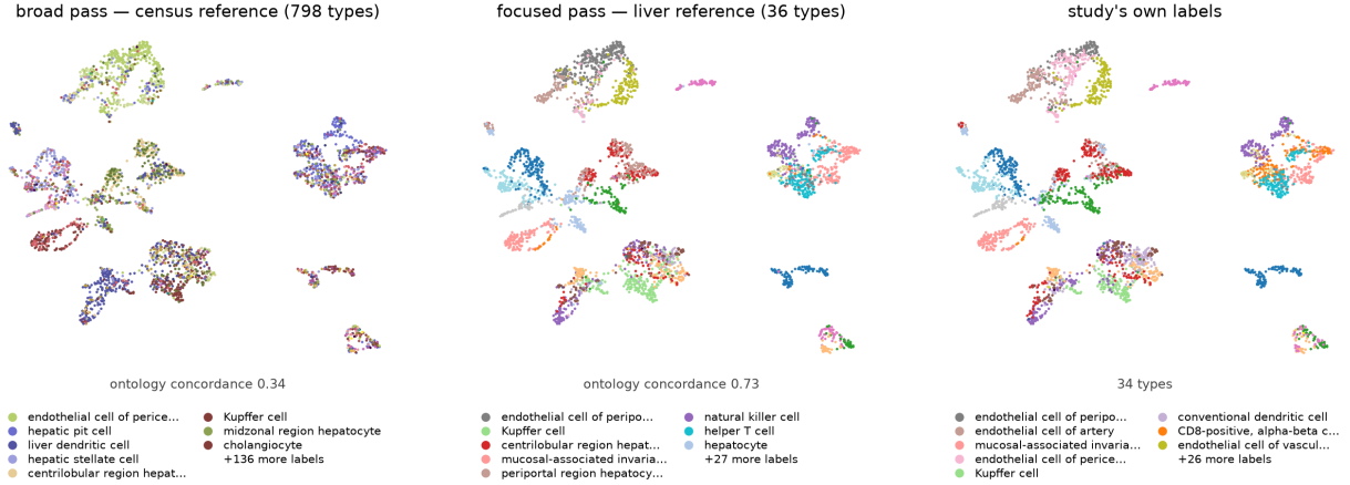
Figure 5. The two passes on the withheld HLiCA liver study (3,396 cells), same UMAP throughout. Left: the shipped census reference spreads 137 of its 798 labels over the query with little correspondence to cluster structure — ontology concordance 0.34 . Its job is to establish that this is liver and route accordingly, not to name subtypes. Middle: a 36-type liver reference trained on the six non-withheld studies re-annotates the same cells at 0.73 , and its labels now track the clusters. Right: the study’s own labels, on the shared palette, for comparison with the middle panel. Both models are leakage-free with respect to this query: the focused reference is trained only on the other six studies (the shipped liver_hlica_v2 includes this study and would score 0.94 here, which is why it is not the model plotted). Abstention is switched off in all panels so the numbers measure labelling rather than coverage; §3.5 covers abstain separately.
