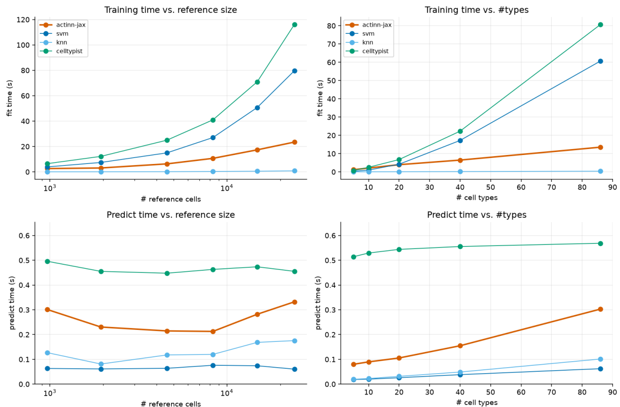
Figure 2. Fit and predict time against reference size and label cardinality. Fit time grows for every trained method; predict time stays sub-second throughout — flat in reference size, and rising to 0.30 s at 86 types.
