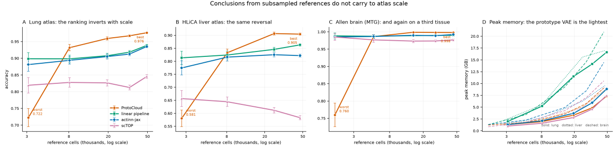
Figure S6. Accuracy and peak memory against reference size, four methods carried to atlas scale on three tissues. A : lung, 3.1k to 49k reference cells. B : the HLiCA liver atlas, 2.7k to 47k. C : Allen brain (MTG), 1.8k to 46k. In each one a prototype VAE moves from worst to best as the reference grows. D : peak memory over all three sweeps. Error bars on A and B are 95% binomial intervals on the query, which grows with the reference (1,035 to 16,398 cells on lung), so they narrow from left to right; each point is a single run.
