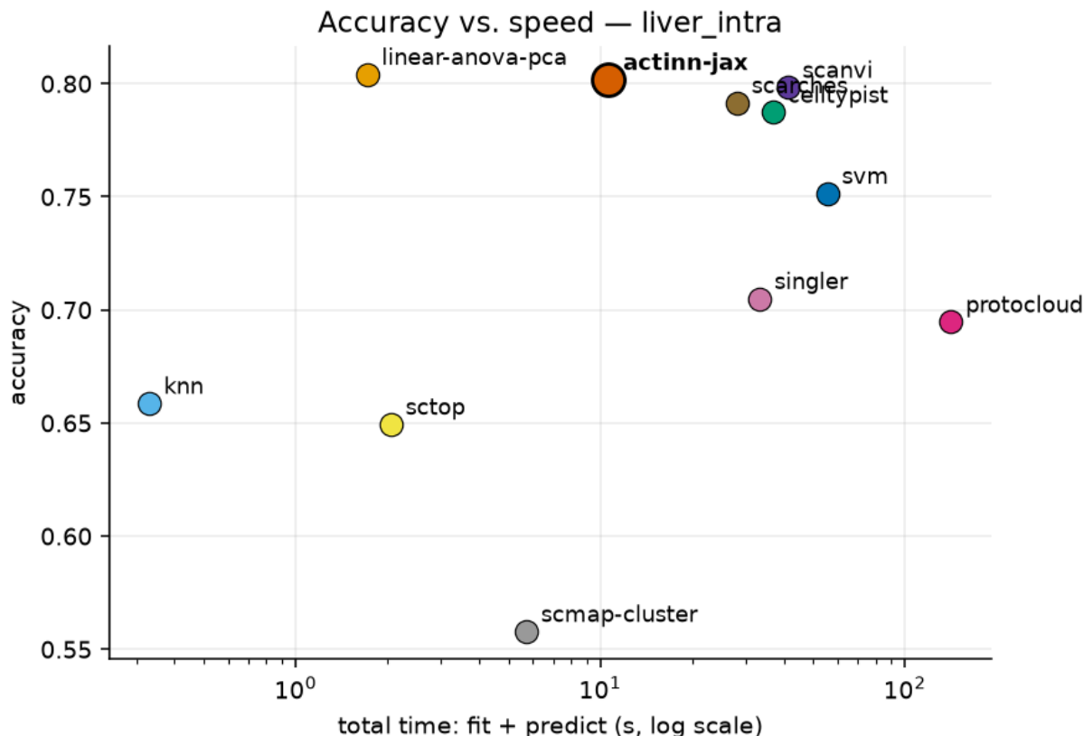
Figure 2. Accuracy against total wall time on liver_intra. The tuned linear pipeline holds the fast-frontier point; actinn-jax sits just inside it at this reference size, and what separates it is visible only on the scaling axes of Figure 3.
