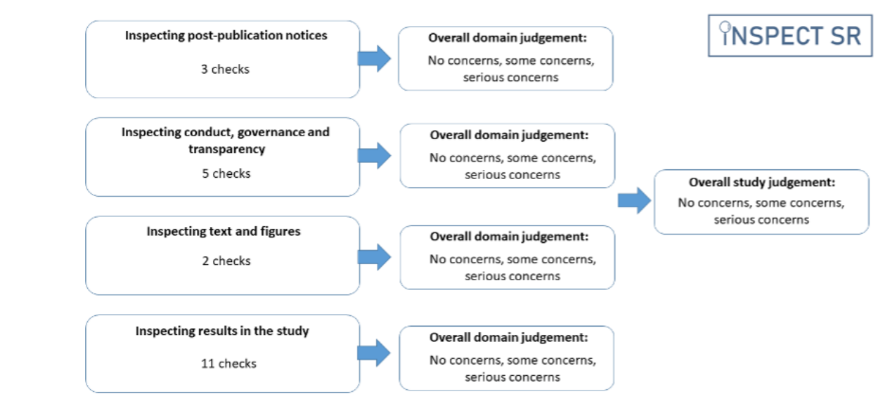
Figure 1: Figure 1: Structure of the INSPECT-SR tool
