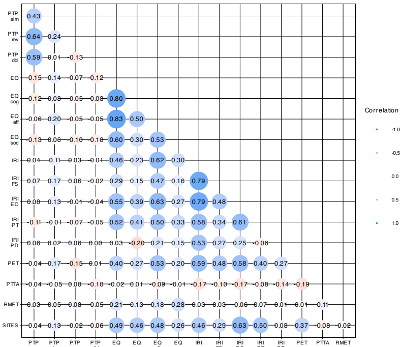
Disattenuated for test-retest reliability (Spearman's rho)
