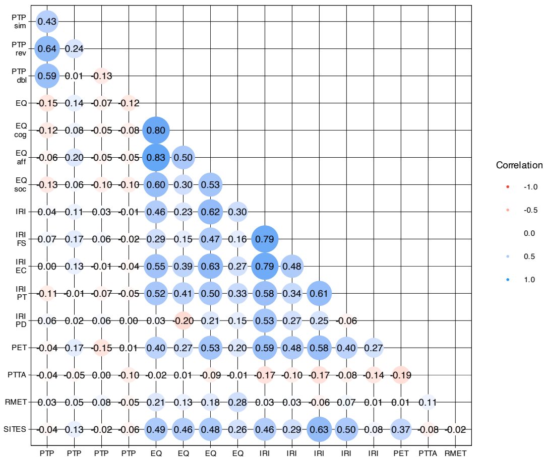
Correlation matrix (Spearman's rho)
