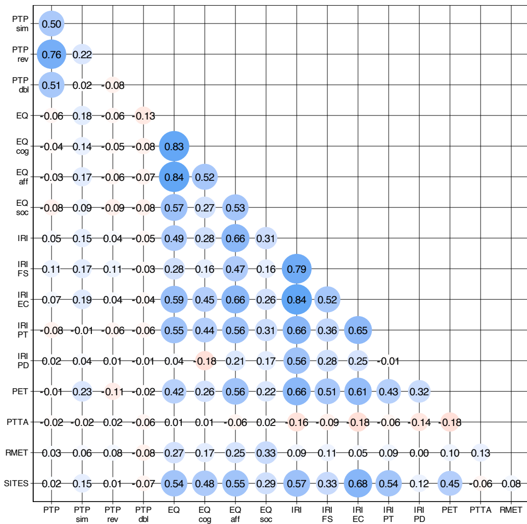
Correlation matrix
