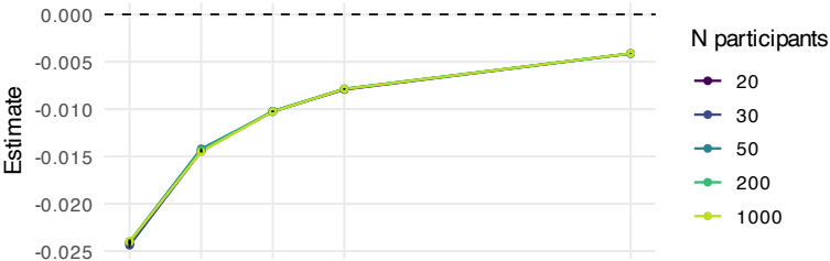
1c. Total bias (sample alpha vs. omega)
