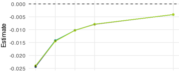
1c. Total bias (sample alpha vs. omega)
