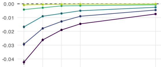
1b. Structural gap (population alpha vs. omega)
