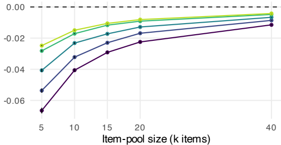
1c. Total bias (sample alpha vs. omega)
