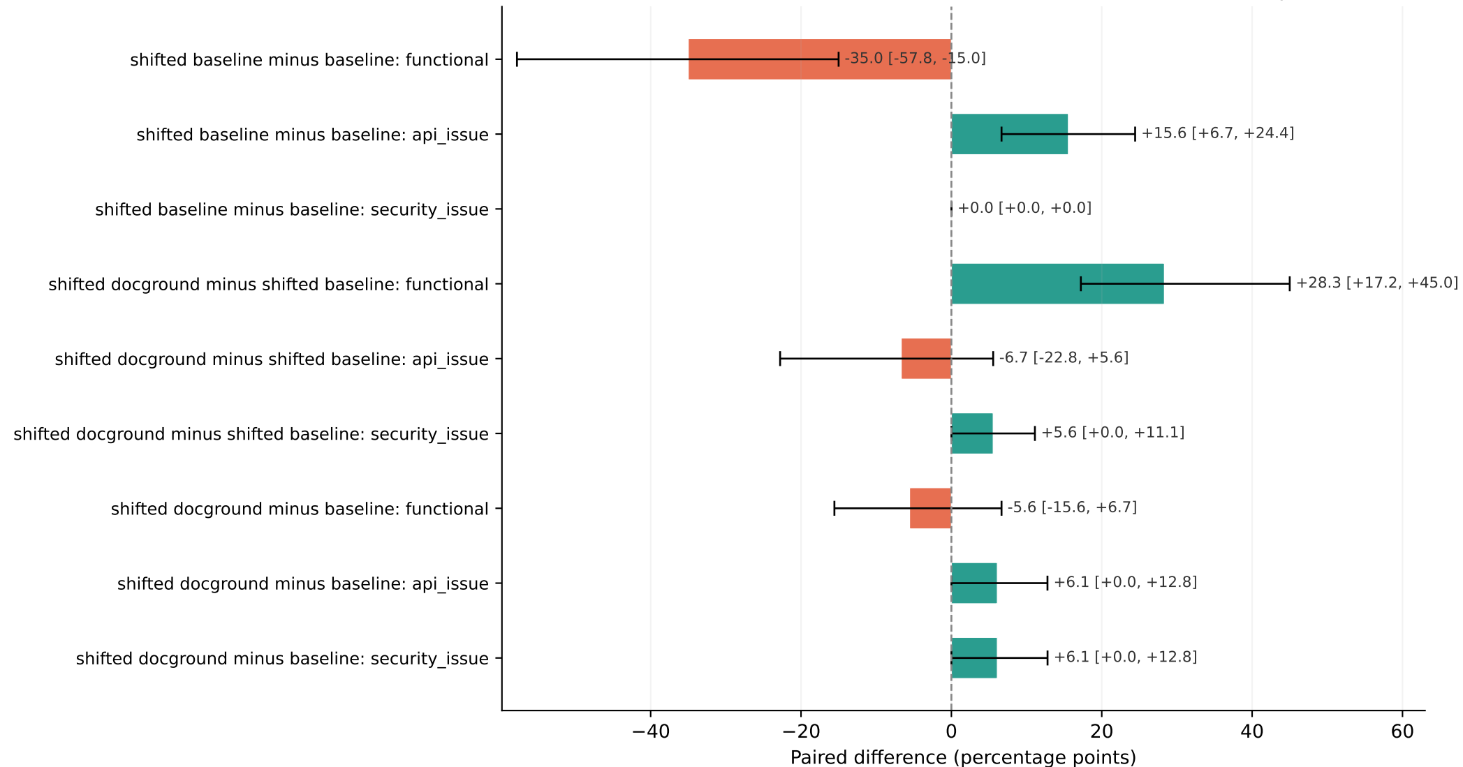
Paired effects (after - before) with 95% task-cluster bootstrap CI
