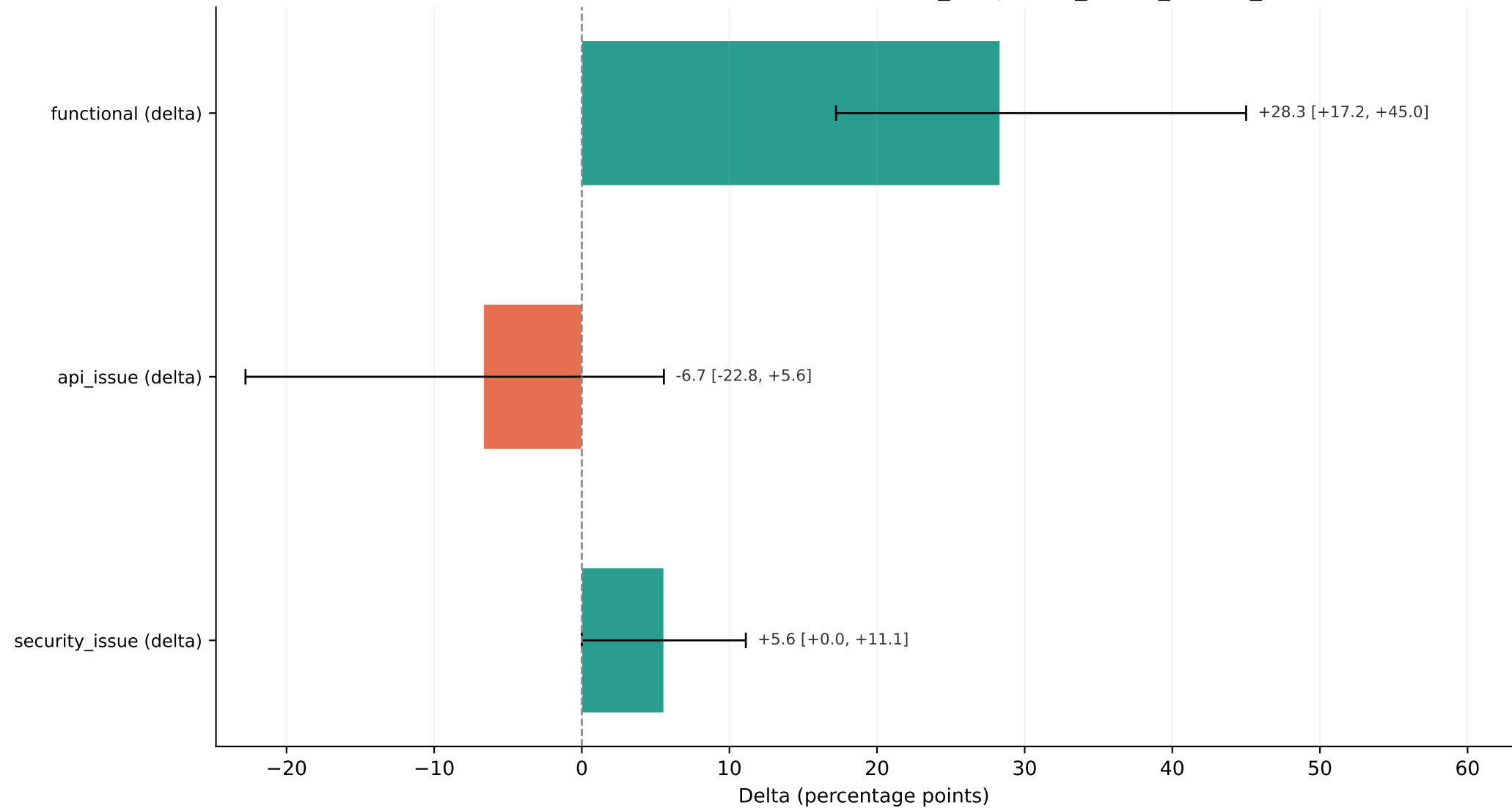
Paired effect (after - before) with 95% CI: shifted_docground_minus_shifted_baseline
