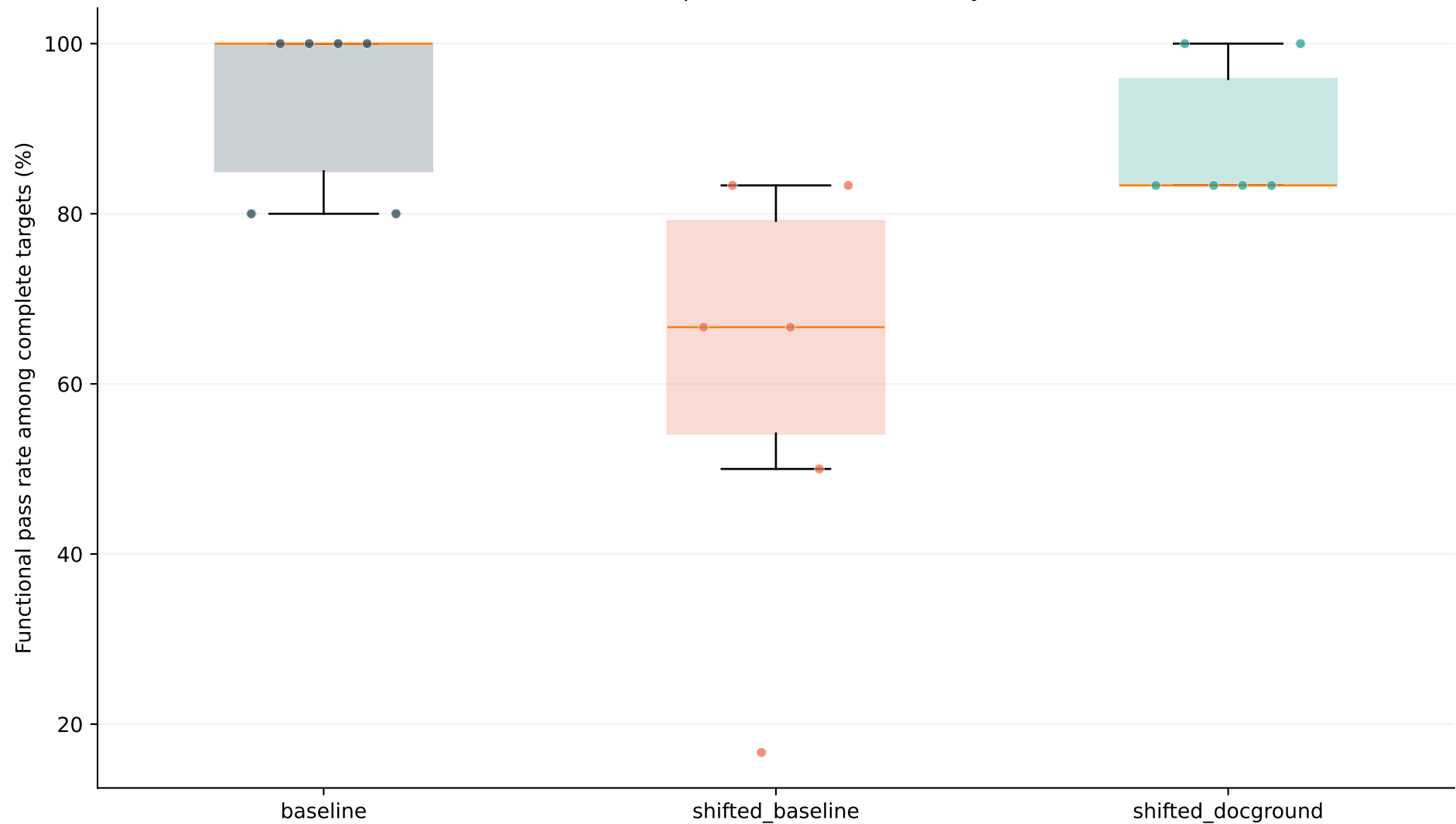
Per-task functional pass rate distribution by condition
