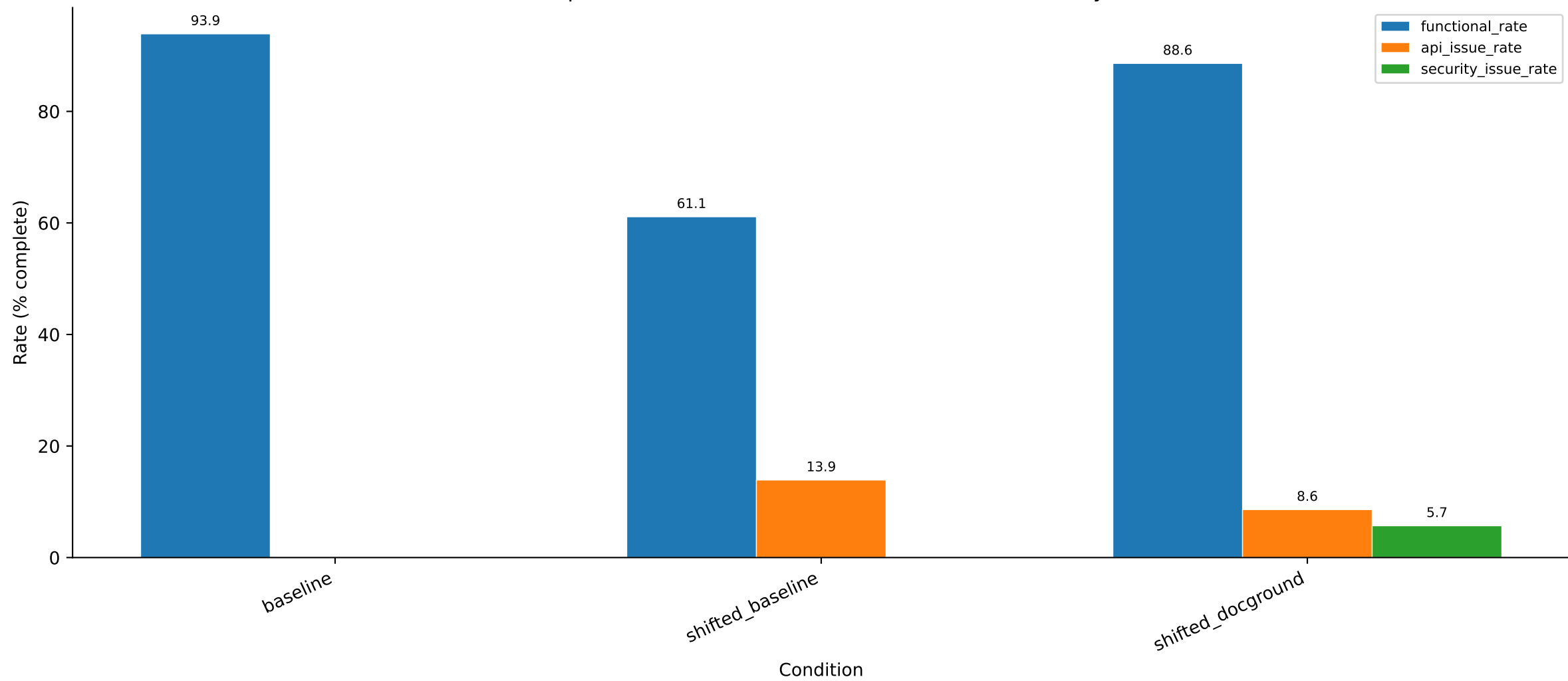
Condition comparison: functional, API-conformance, and security-issue rates
