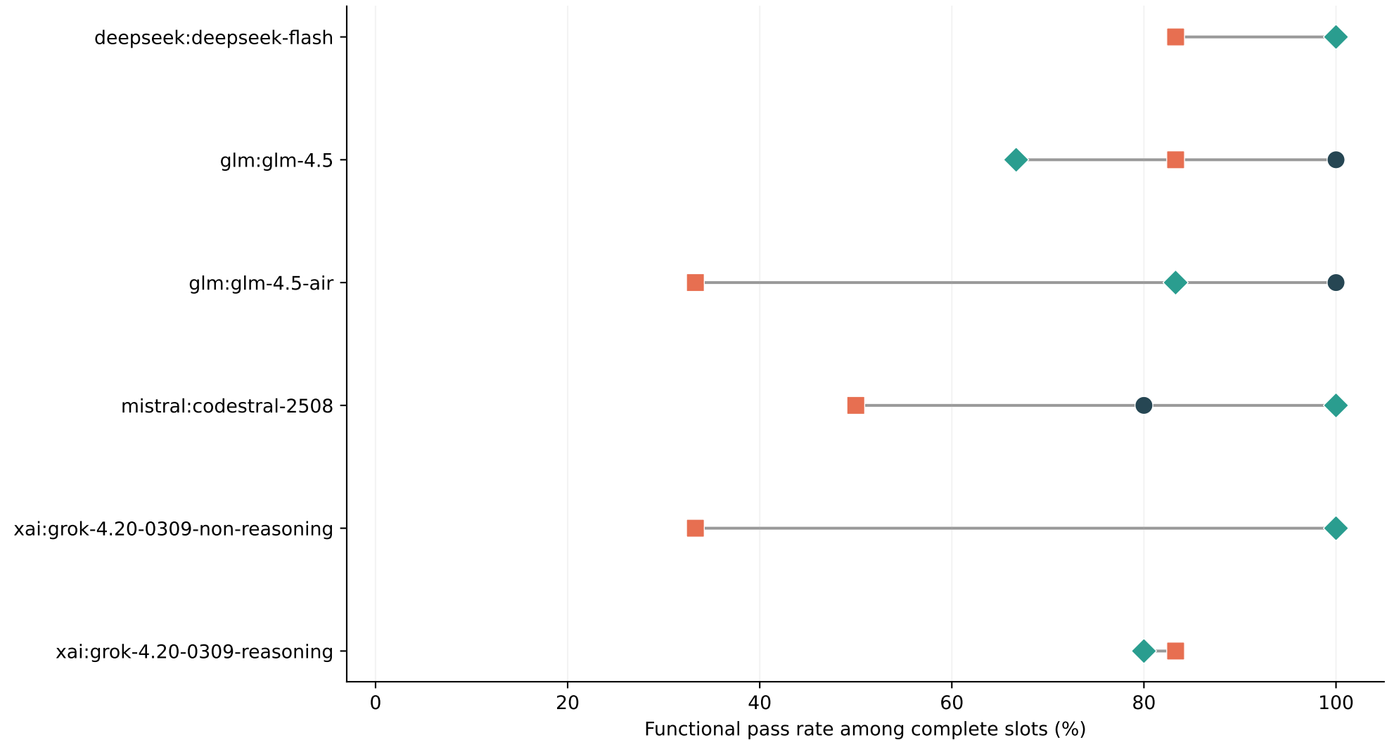
Functional pass rate by model and condition
