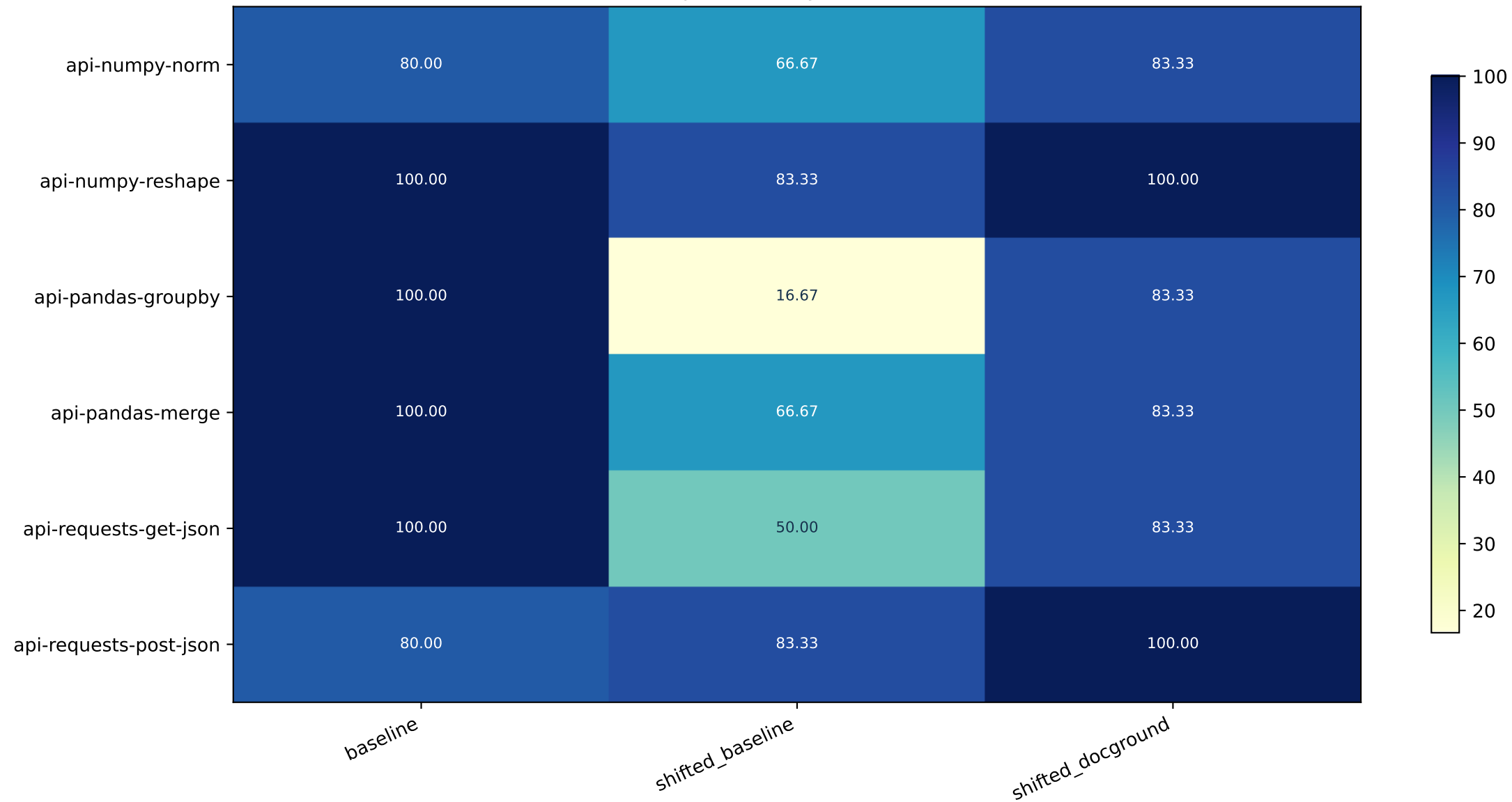
Functional pass rate by task and condition
