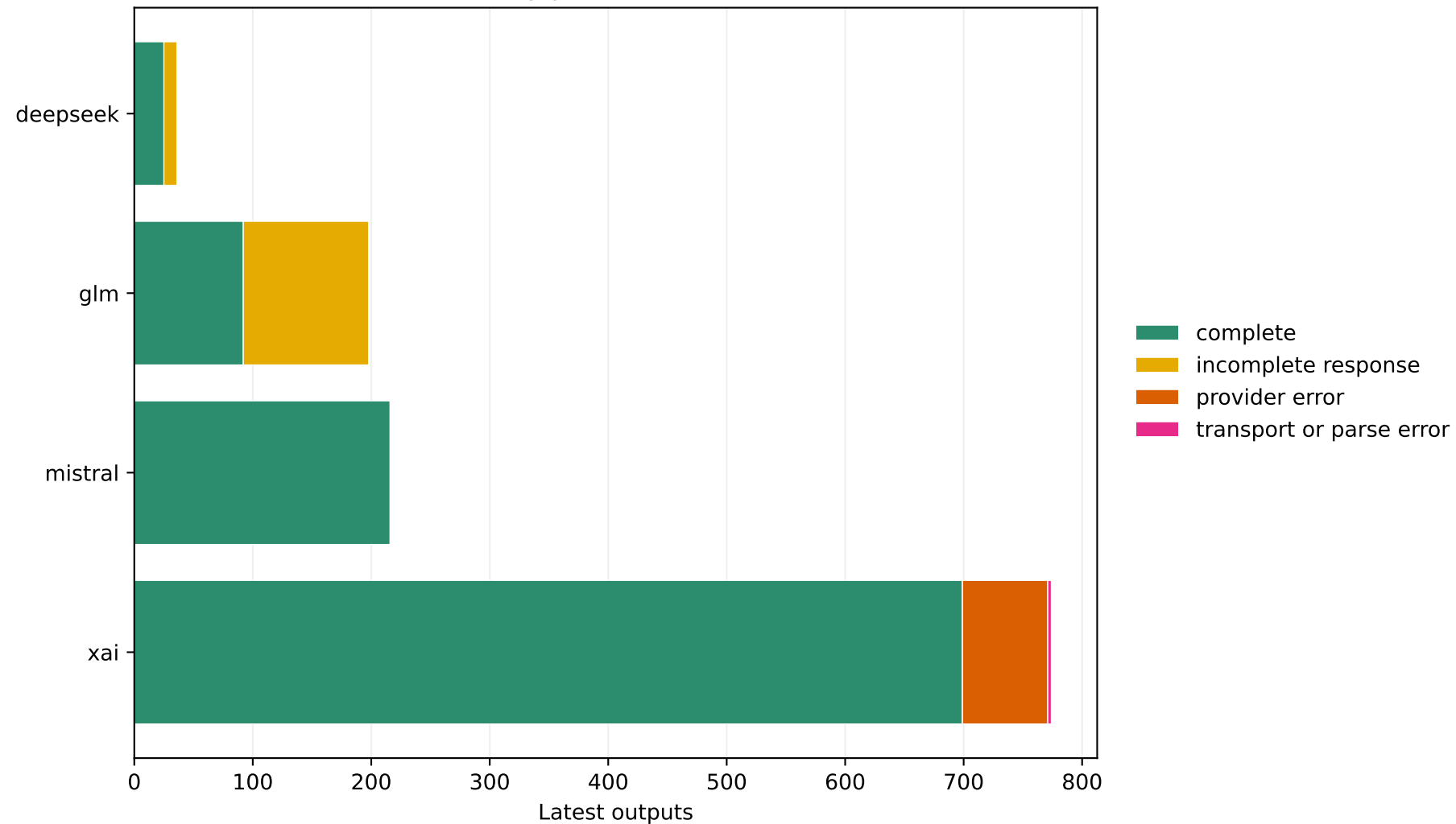
Generation status by provider. 6 task execution audit
