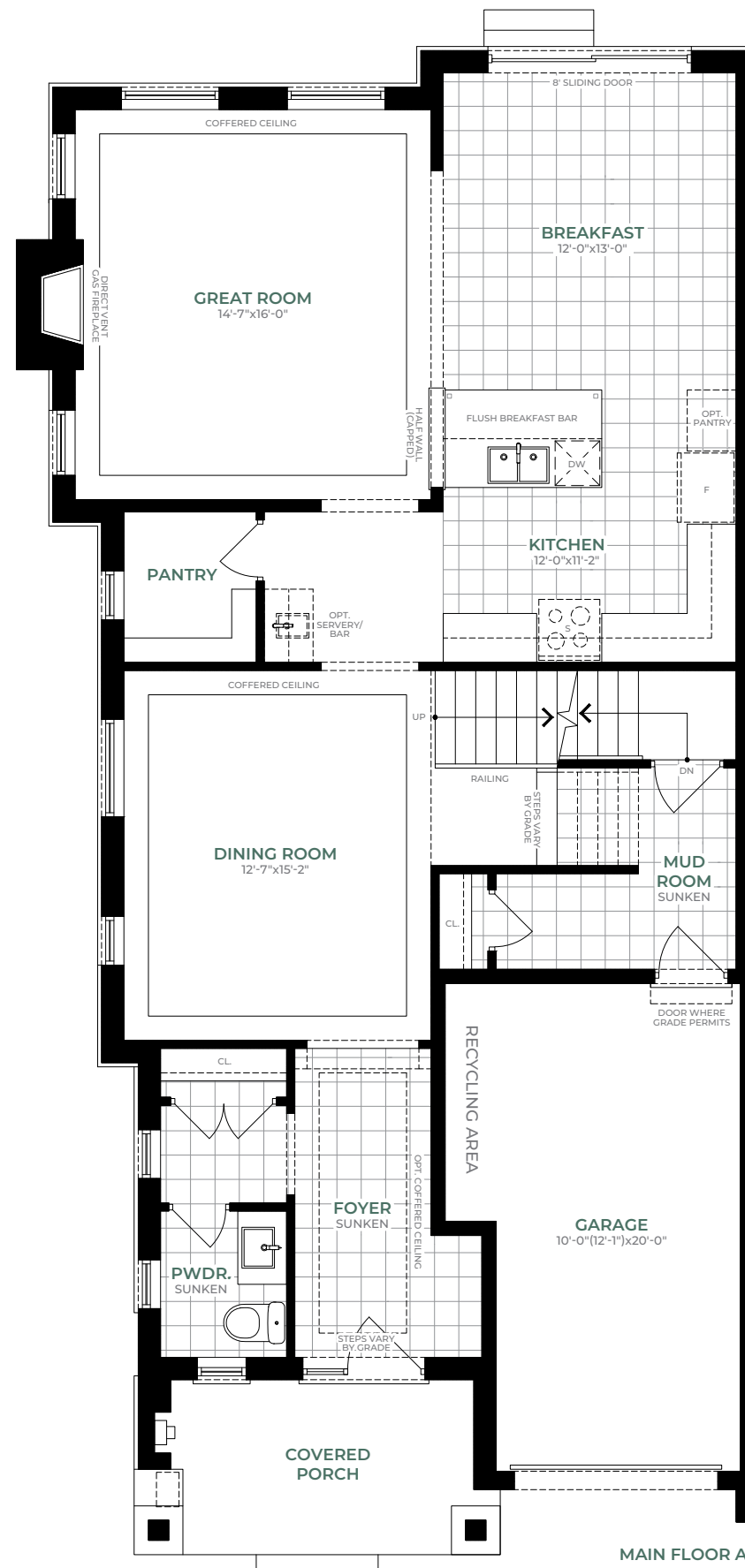
MAIN FLOOR A
