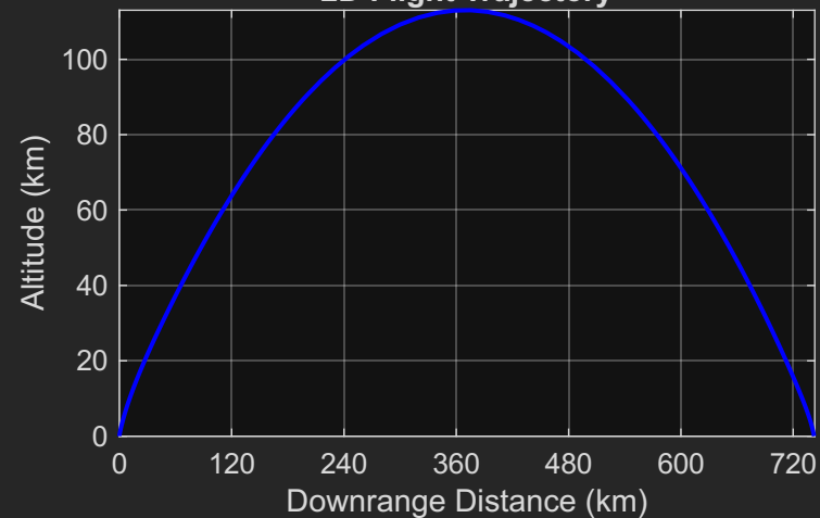
2D Flight Trajectory
