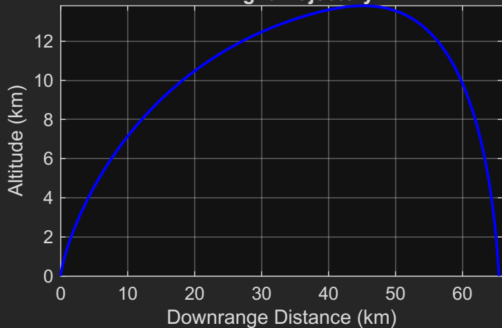
2D Flight Trajectory
