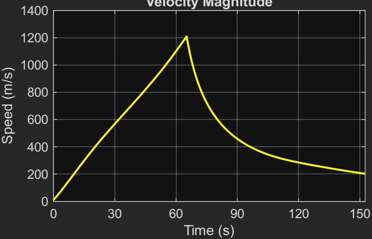
Velocity Magnitude
