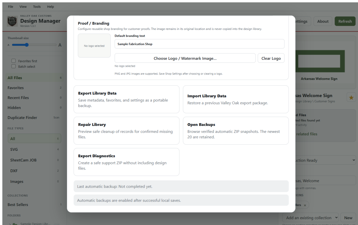
Backup and maintenance controls.
