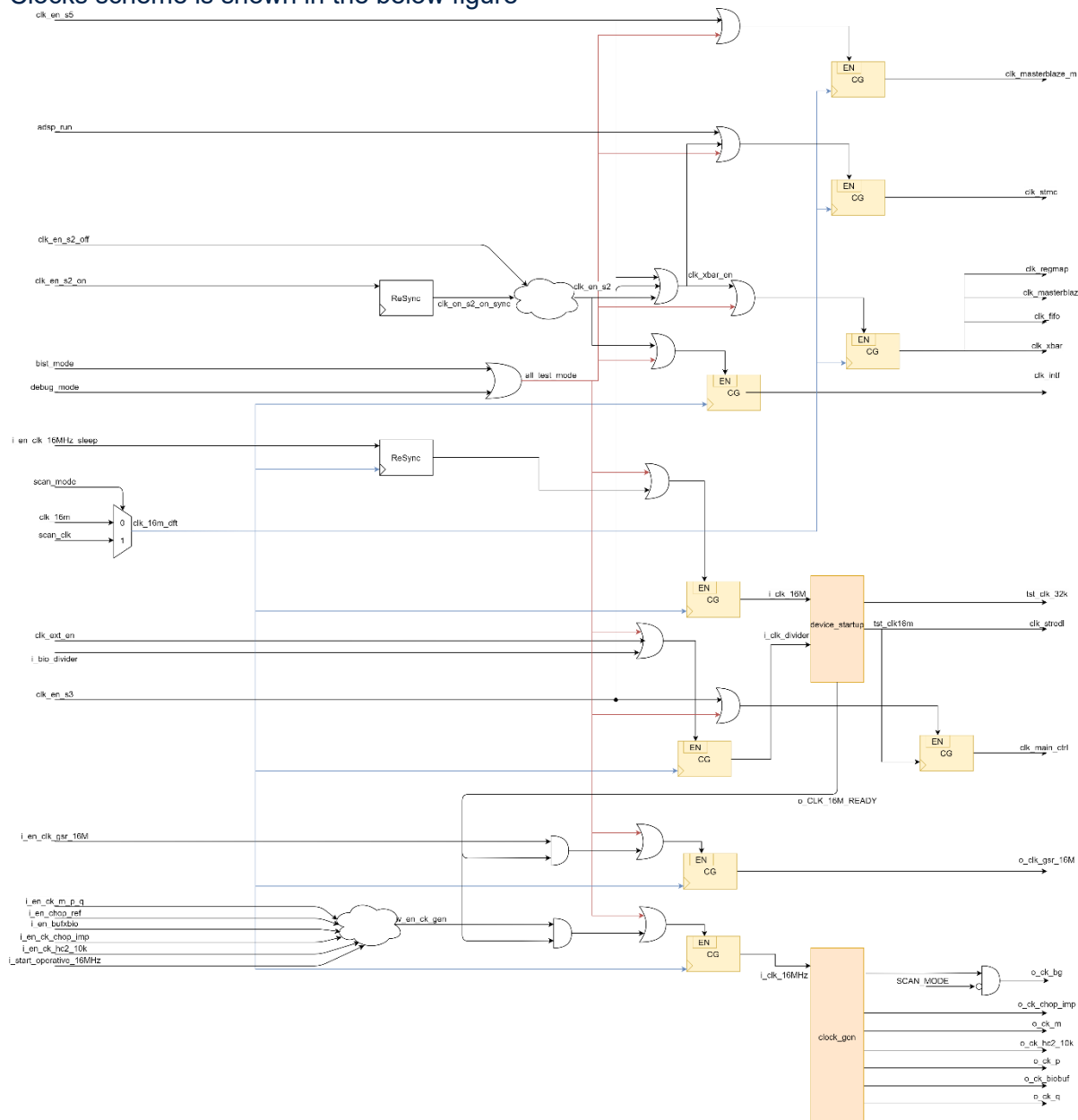
Figure 9: Clocks Scheme
