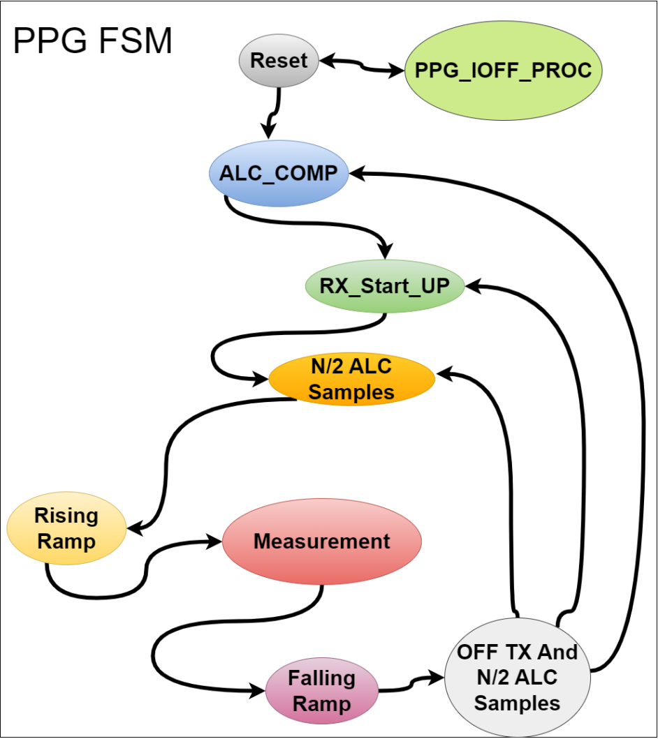
Figure 12: PPG FSM State Diagram
