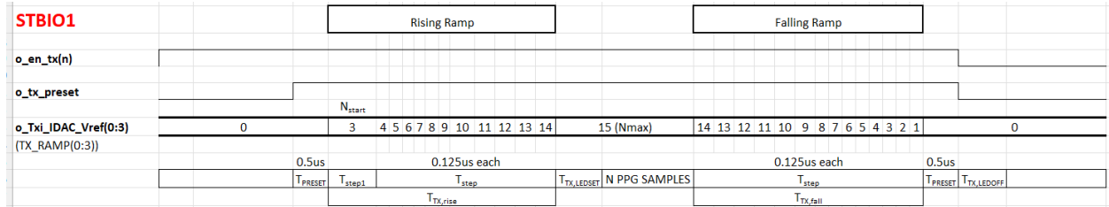
Figure 15: Digital Ramp Time Diagram
