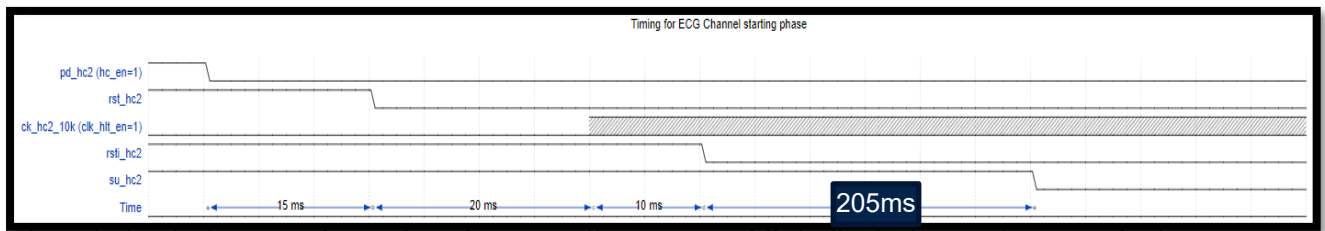
Figure 6: ECG start up phase with chopper clock
