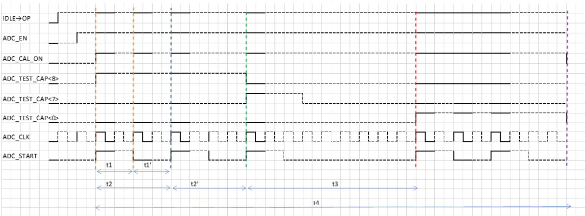
Figure 4: ADC Calibration Phase Time Diagram
