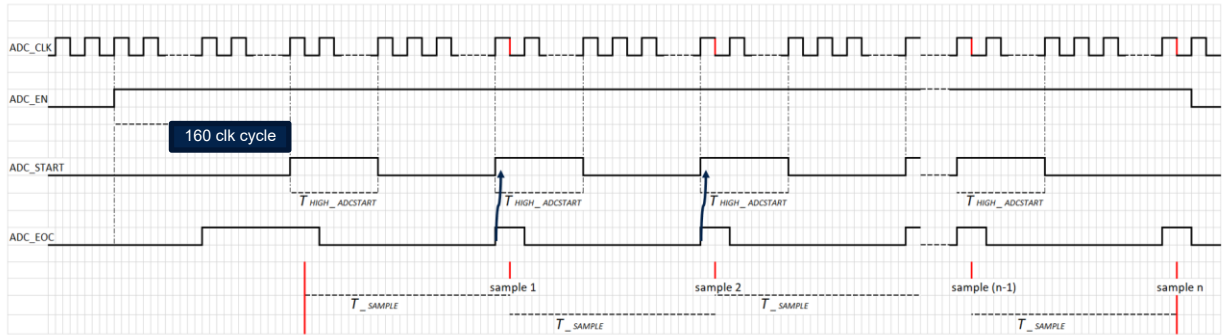
Figure 3: ADC PHGen Time Diagram:
