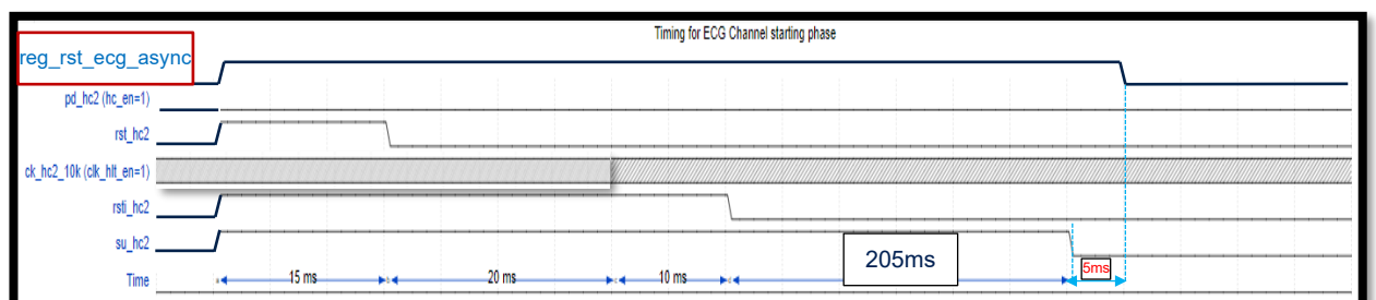
Figure 7: ECG Start-UP phase with asynch reset
