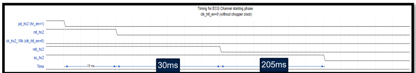
Figure 8: ECG Start Up phase with no Chopper Clock
