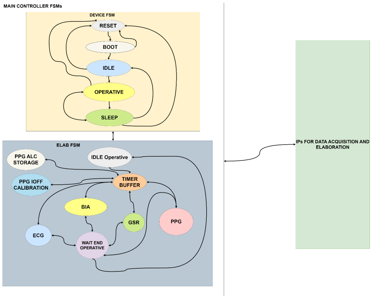
Figure 2: Main Controller FSM Diagram
