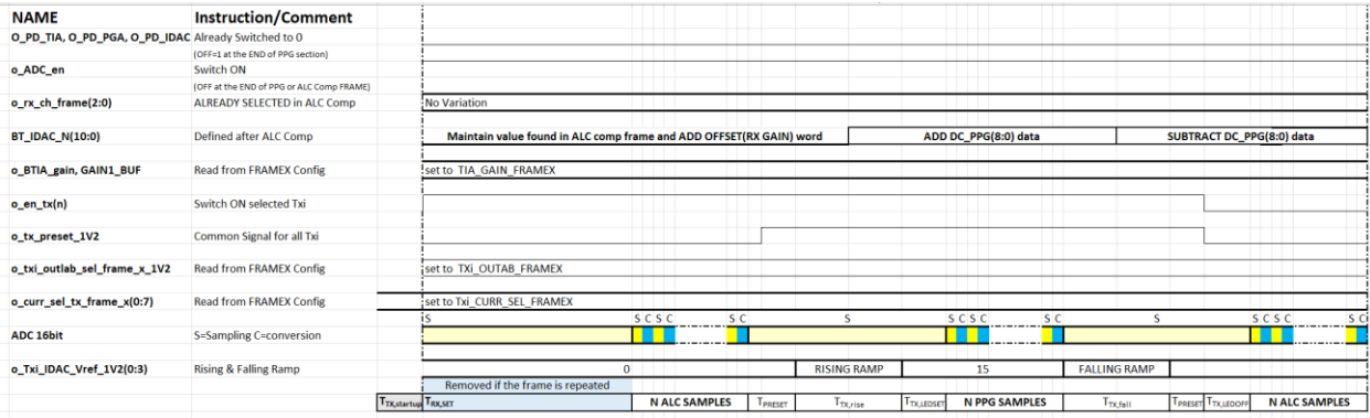
Figure 13: PPG Time Diagram
