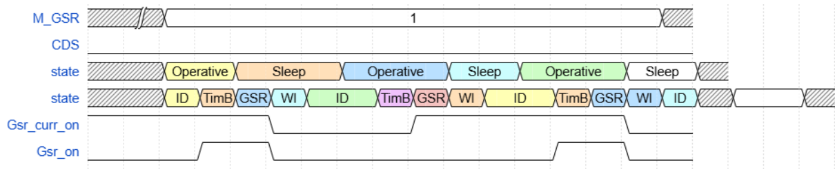
Figure 10: GSR with CDS Disabled and m\_GSR set to 1
