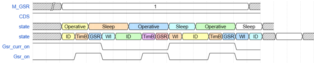
Figure 11: GSR with CDS Enabled with m\_gsr set to 1
