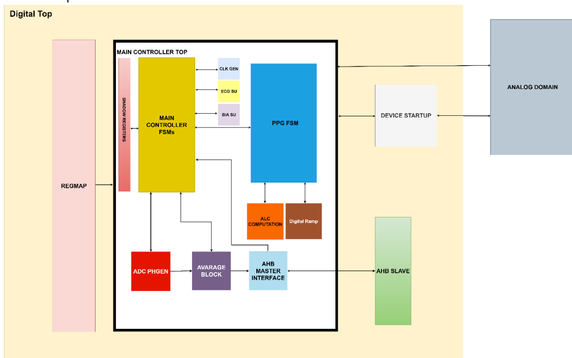
Figure 1: Main Controller Ip Block Diagram
