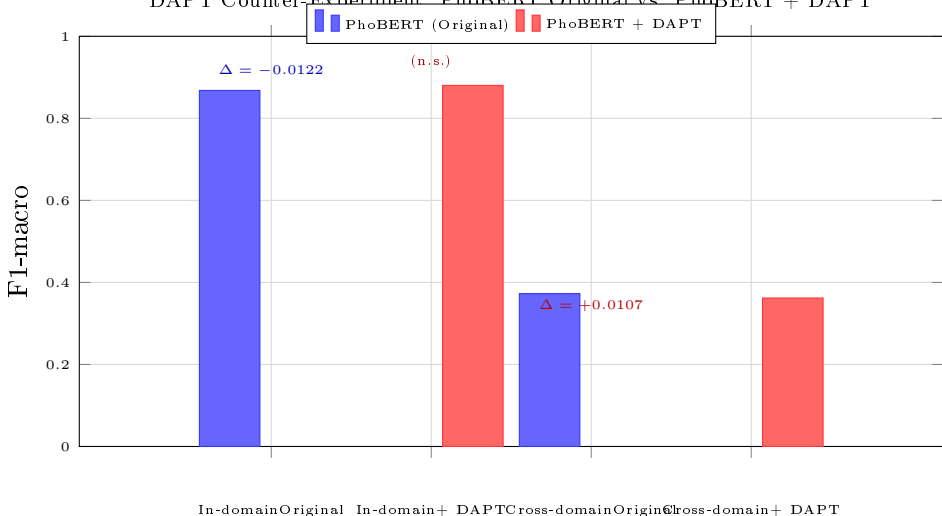
DAPT Counter-Experiment: PhoBERT Original vs. PhoBERT + DAPT
