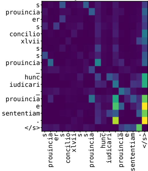
Query self-attention
