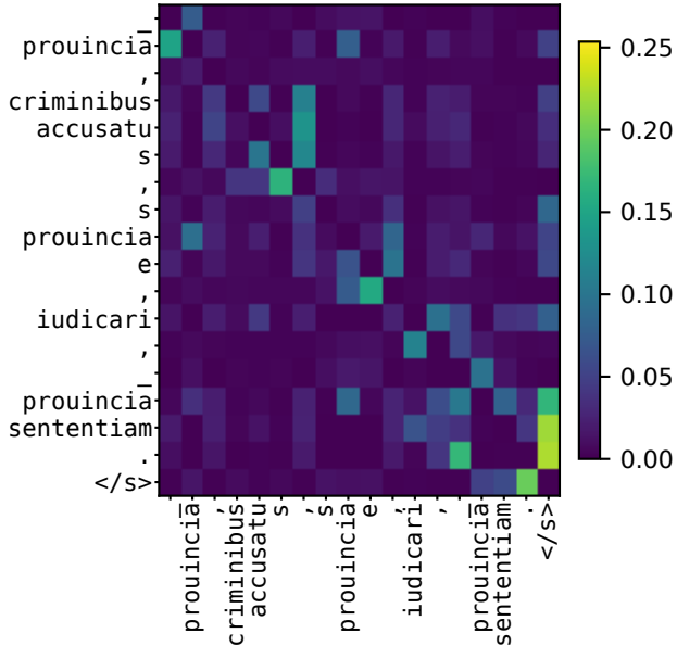
Candidate self-attention
