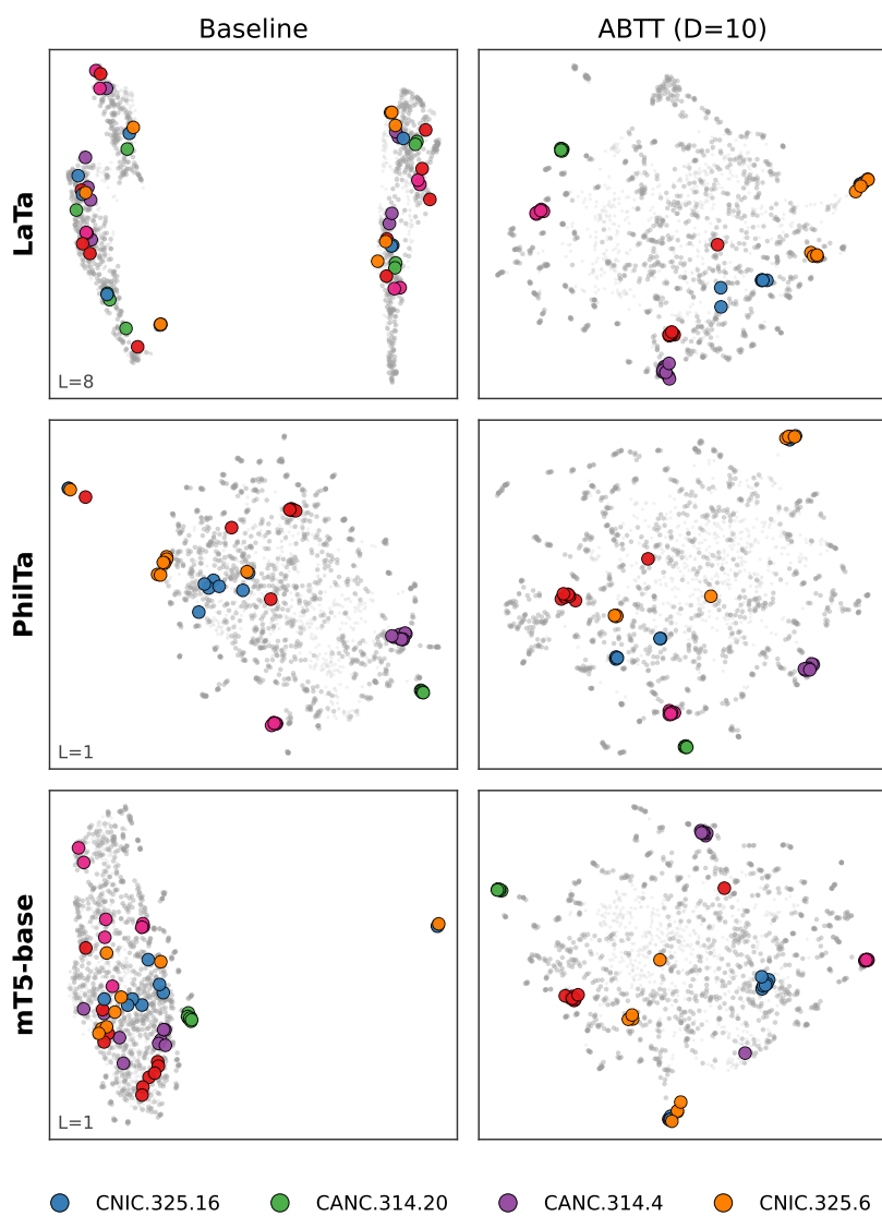
Figure 9: UMAP projections with the same configuration as Figure 8. The same cluster-tightening pattern appears under a different projection method.
