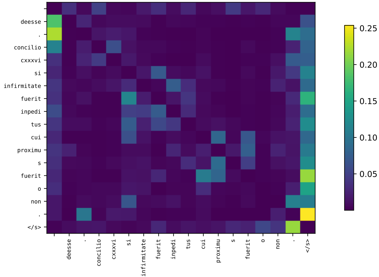
Candidate Self-Attention
