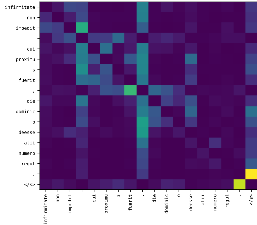
Query Self-Attention
