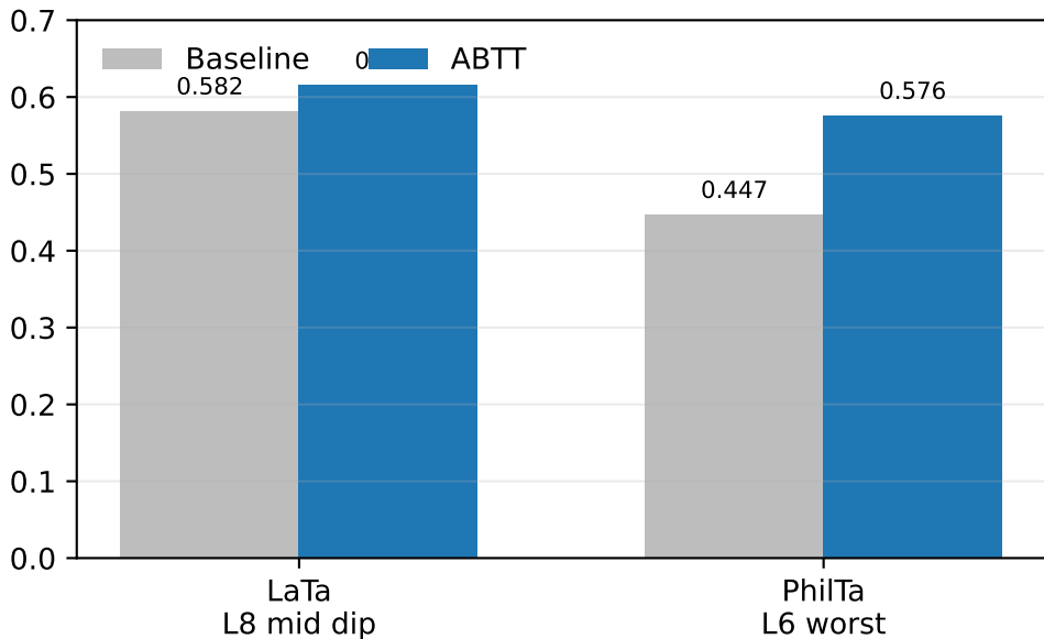
Content-token share
