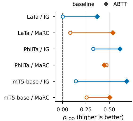
Figure 7: Leave-one-out rank correlation \rho_{\text{LOO}} at the predeclared operational attribution layers, for integrated gradients (IG) and retrieval-adapted MaRC. Each line connects the baseline and ABTT variants of one model-method cell. ABTT raises \rho_{\text{LOO}} in five of the six cells; the sixth, PhilTa MaRC, moves from 0.469 to 0.445, a tie within two standard errors (Table 23). Secondary metrics: Table 24.
