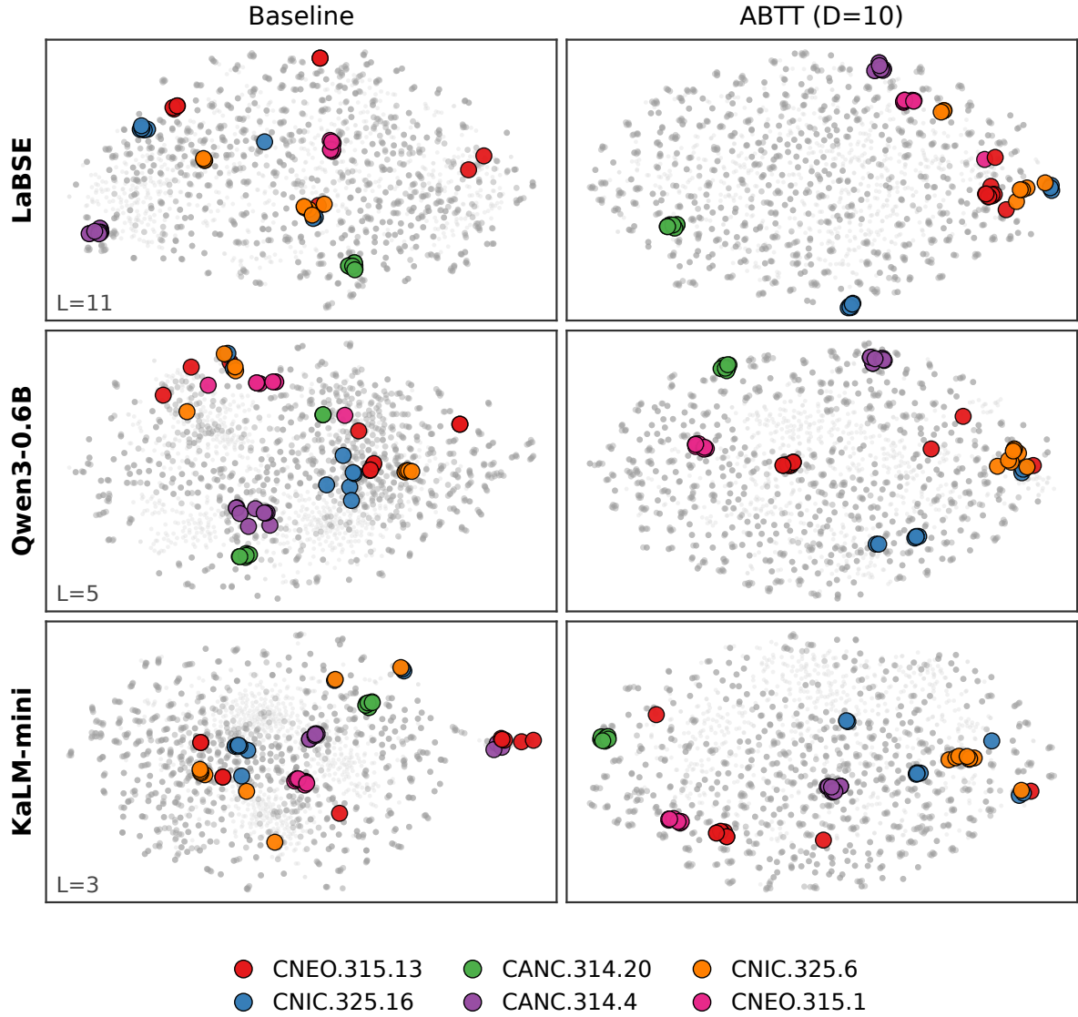
Figure 13: t-SNE projections of all 1,705 manuscript witnesses for LaBSE, Qwen3-0.6B, and KaLM-mini under the layer rule of Figure 11: the layer with the highest training-set DirAcc@1 under ABTT, printed in each panel and equal to the Task B ABTT layer in Table 9. Columns compare baseline mean pooling with ABTT-only using D = 10 . Colors mark the same six largest directories as Figure 11.
