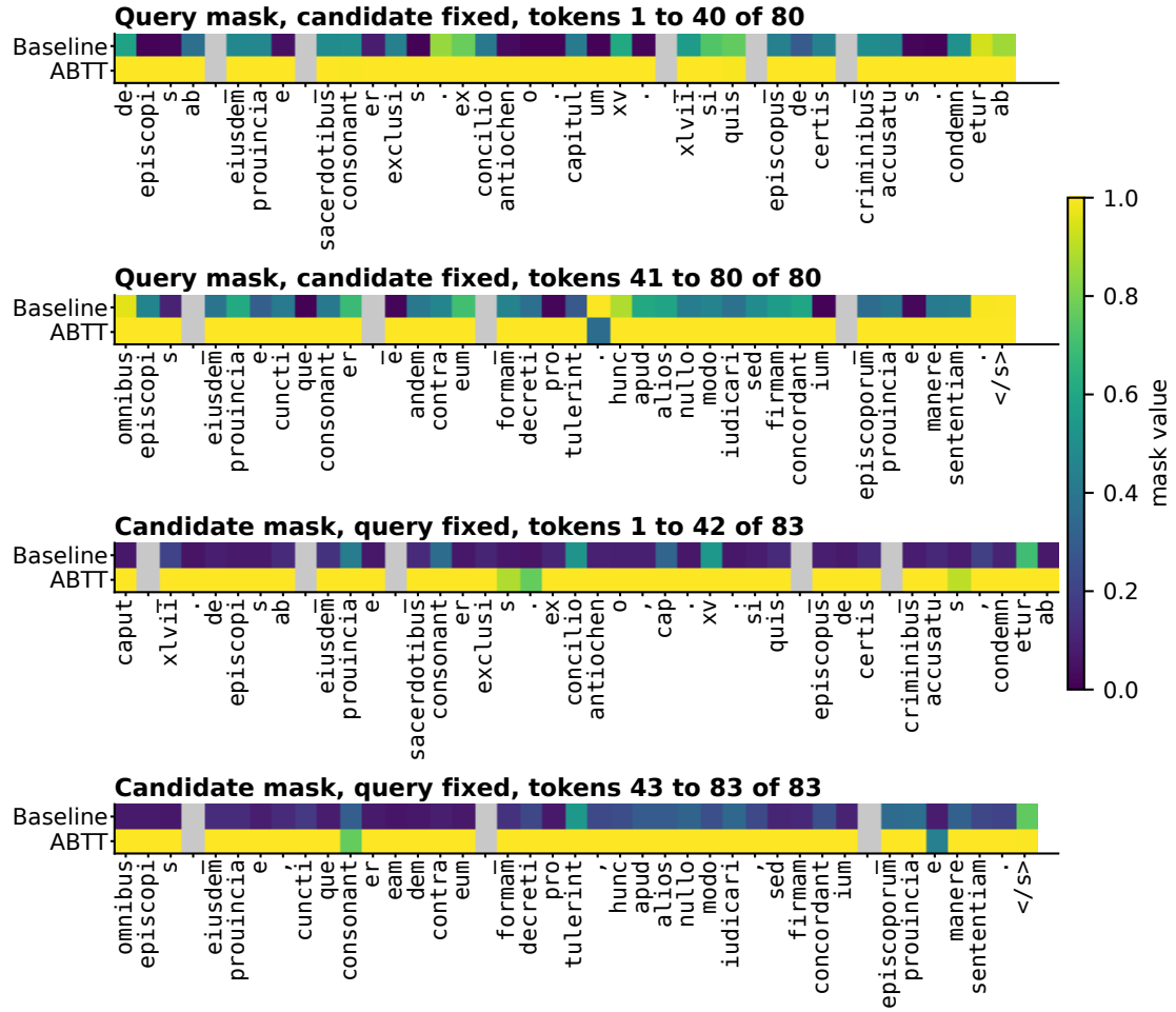
Figure 10: Retrieval-adapted MaRC masks at PhilTa layer 6 for the same demonstration pair as Figure 8, which is outside the 200 evaluated pairs. The upper two strips give the mask on the query with the candidate fixed, and the lower two the mask on the candidate with the query fixed; each sequence wraps onto two strips. In every strip the Baseline row uses the raw cosine target and the ABTT row the ABTT-corrected cosine target. Gray cells are non-content positions, frozen at zero.
