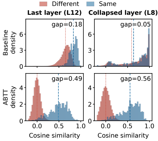
Figure 6: Cosine similarity distributions for PhilTa at the last layer and at its collapsed retrieval layer, before and after ABTT. Equivalent pairs share a directory (Same in the legend); non-equivalent pairs do not (Different). The collapsed retrieval layer is layer 8, chosen by a train-only rule (highest training-set AUROC within 30 to 70 percent of encoder depth, layers 4 to 8), so the panel understates the collapse rather than selecting its worst case; its test AUROC is 0.542, close to chance. Two other PhilTa layers carry other meanings and are not shown here: the most anisotropic layer under the top-PC rule of Appendix B is layer 6, and the lowest baseline test AUROC, 0.538, falls at layer 10. Before ABTT the two distributions sit almost on top of each other, and ABTT separates them.
