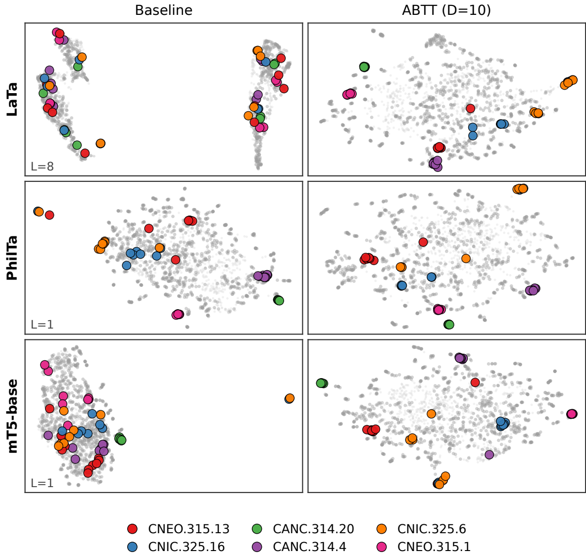
Figure 12: UMAP projections with the same configuration as Figure 11. The same cluster-tightening pattern appears under a different projection method.
