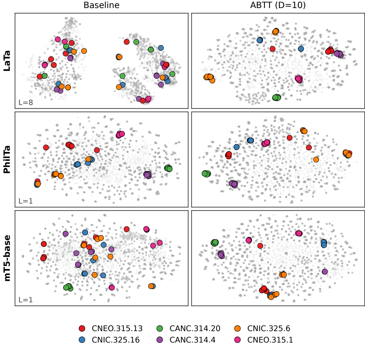
Figure 11: t-SNE projections of all 1,705 manuscript witnesses for LaTa, PhilTa, and mT5-base, each at the layer chosen on the train split: the layer with the highest training-set \text{DirAcc}@1 under ABTT, printed in each panel as L and equal to the Task B ABTT layer in Table 9. Columns compare baseline mean pooling with ABTT-only using D = 10 , fit on the training embeddings. Colors mark the six largest directories; other witnesses of directories with at least two witnesses are mid gray, and singletons light gray. The silhouette scores in Appendix L are computed in these two-dimensional coordinates over the 1,160 winnable witnesses, those whose directory has at least two witnesses.
