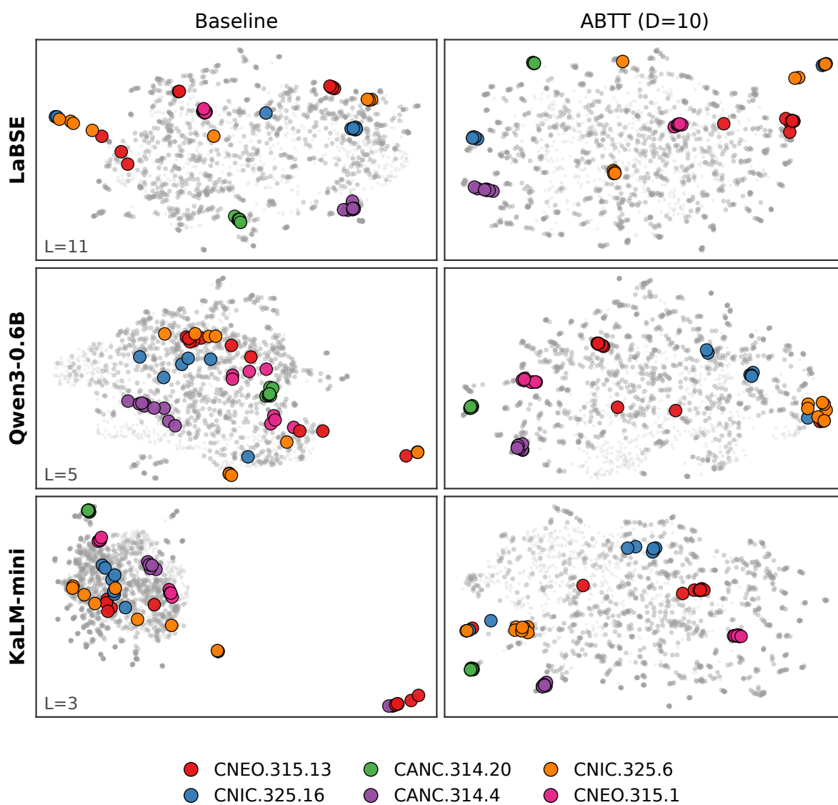
Figure 14: UMAP projections matching Figure 13. The cluster-tightening pattern appears under a second projection method.
