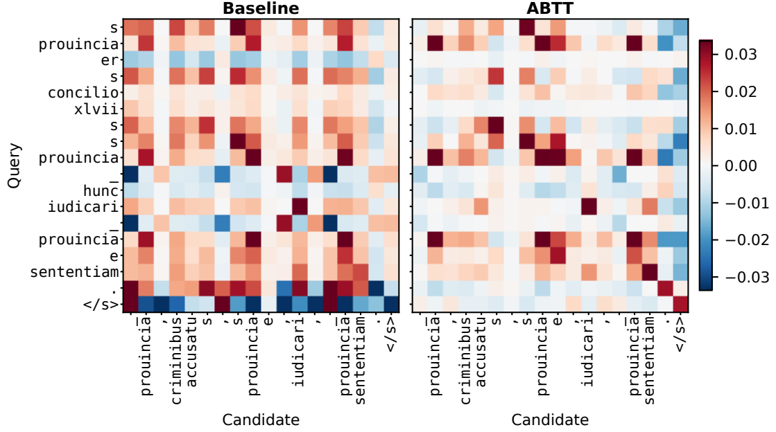
Figure 8: Derived pairwise heatmap for one PhilTa retrieval pair, at PhilTa layer 6, its most anisotropic layer (the layer of the mechanism check in Appendix I), not the operational layer of Table 23; a demonstration pair chosen because ABTT reverses the baseline decision, outside the 200 evaluated pairs. The left panel shows the baseline representation and the right panel shows the same example after ABTT. Both axes use original decoded tokens: the 18 query and 18 candidate tokens with the largest integrated-gradient magnitude under either representation. Cell values combine token-token cosine similarity with single-sequence integrated-gradient scores.
