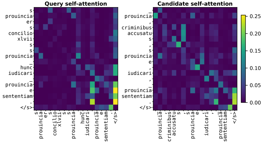
Figure 9: Companion self-attention maps at PhilTa layer 6 for the same demonstration pair as Figure 8, which is outside the 200 evaluated pairs. ABTT is applied after encoding, so attention is included only as supporting context.
