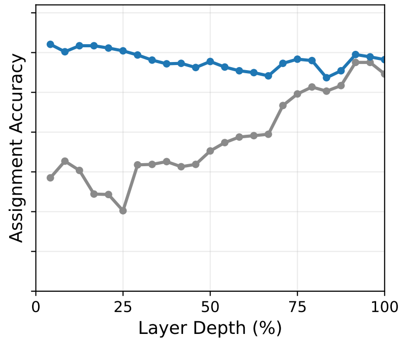
KaLM-mini
