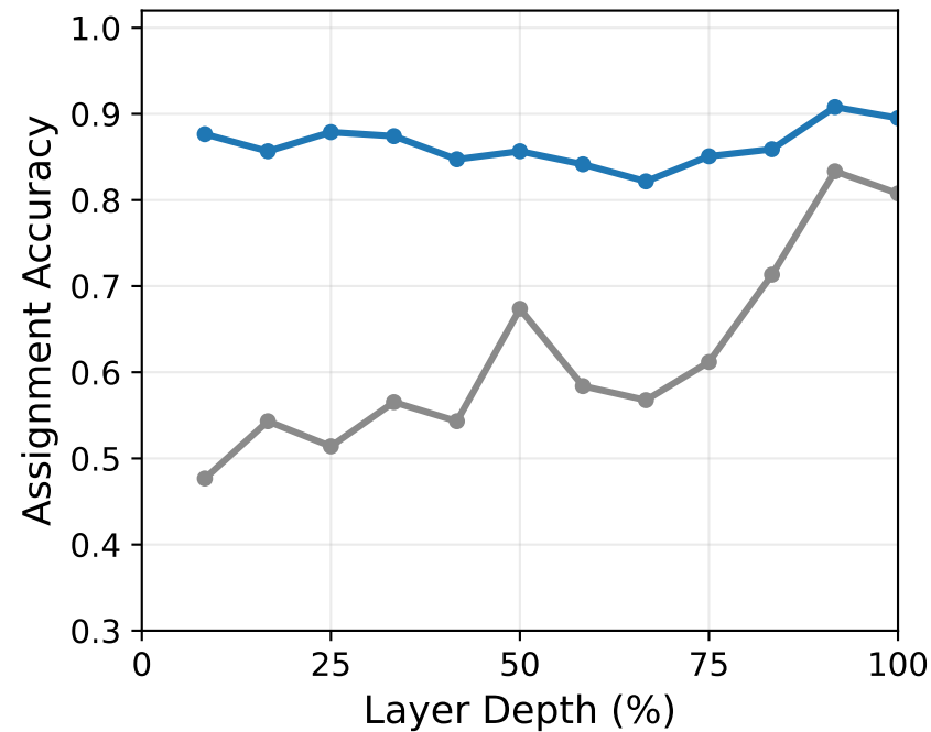
LaBSE
