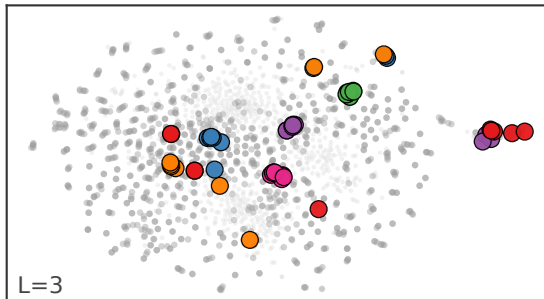
KaLM-mini
