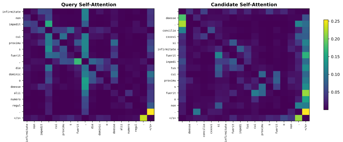
Figure 8: Companion self-attention maps for the same PhilTa example as Figure 7. ABTT is applied after encoding, so attention is included only as supporting context.
