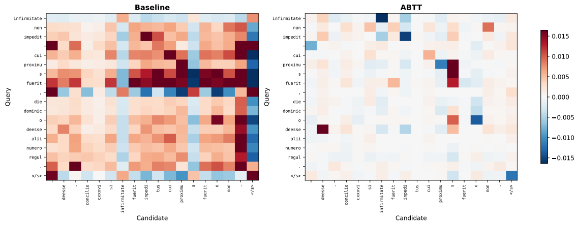
Figure 7: Derived pairwise heatmap for one PhilTa retrieval case. The left panel shows the baseline representation and the right panel shows the same example after ABTT. Both axes use original decoded tokens. Cell values combine token-token cosine similarity with single-sequence integrated-gradient scores.
