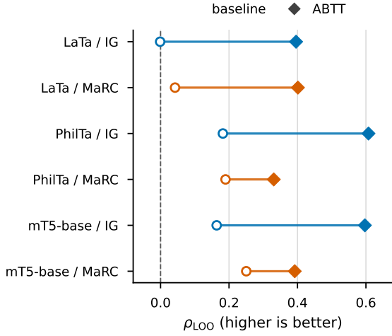
Figure 6: \rho_{LOO} foreground view for the main candidate-attribution result. Each line connects the baseline and ABTT variants for one model-method cell at the predeclared operational attribution layer. ABTT improves the leave-one-out rank-correlation signal in all six cells; Table 4 shows the ERASER-style disagreements which qualify this narrower faithfulness claim.
