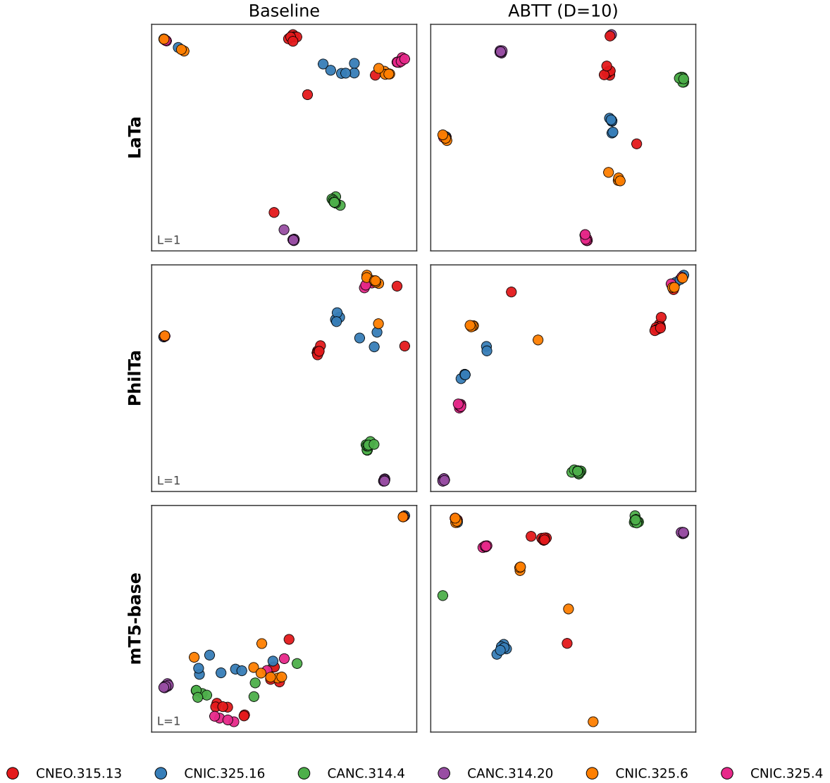
Figure 5: UMAP projections with the same configuration as Figure 4. The same cluster-tightening pattern appears under a different projection method.
