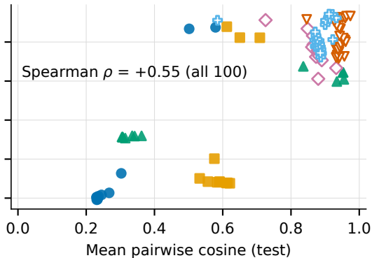
(b) Mean pairwise cosine
