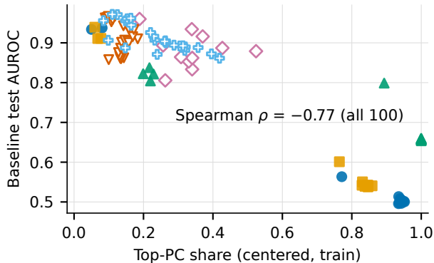
(a) Top-PC share
