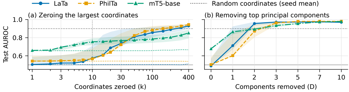
Figure 3: Test ranking AUROC at the 26 collapsed layers of LaTa (10 layers), PhilTa (9) and mT5-base (7); lines: median over a model’s collapsed layers; bands: their range; dashed line: AUROC 0.90. (a) Zeroing the k coordinates of largest mean absolute value; dotted: k random coordinates (mean of five draws). Up to k = 10 (vertical line) the best layer reaches 0.794. (b) Removing the top D principal components ( D = 0 : centering only; ticks follow the selection grid, not evenly spaced in D ). From D = 3 every layer passes 0.90. All fits use training embeddings.
