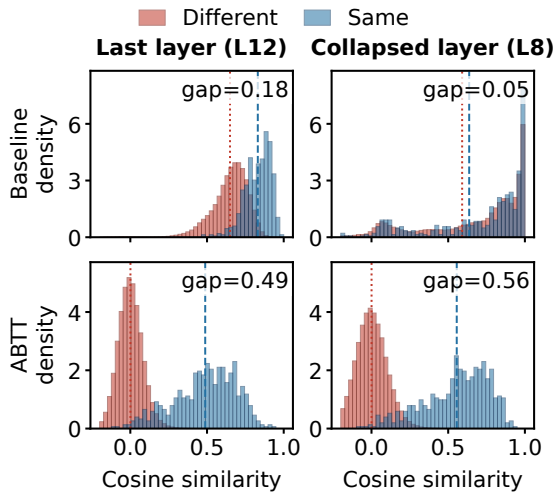
Figure 6: Cosine similarity distributions for PhilTa at its last layer and at the collapsed layer 8 (test AUROC 0.542, close to chance), before and after ABTT. Same: pairs that share a directory; Different: pairs that do not; dashed and dotted vertical lines: the Same and Different means; gap: their difference. Layer 8 has the highest training AUROC of PhilTa’s layers 4 to 8 (30 to 70% of depth), all of them collapsed, so it is not PhilTa’s worst layer: that is layer 10, at baseline test AUROC 0.538. Before ABTT the two distributions sit almost on top of each other, and ABTT separates them.
