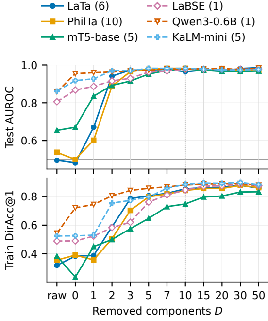
Figure 9: Test ranking AUROC (top) and training DirAcc@1 as a fraction (bottom) against the number D of removed principal components, one line per model at its lowest-AUROC baseline layer (in parentheses in the legend). The horizontal axis is categorical: raw is the uncorrected vector, D = 0 is centering on the training mean alone, and the ticks are not evenly spaced in D . ABTT is fit on training embeddings only; the dotted vertical line marks D = 10 , the top of the selection grid, and the gray horizontal line chance (AUROC 0.5). Filled markers and solid lines: T5 encoders; hollow markers and dashed lines: embedding-trained models. At the plotted T5 layers one component restores part of the ranking. LaTa and PhilTa recover nearly all of it with two or three components; mT5-base keeps improving up to ten.
