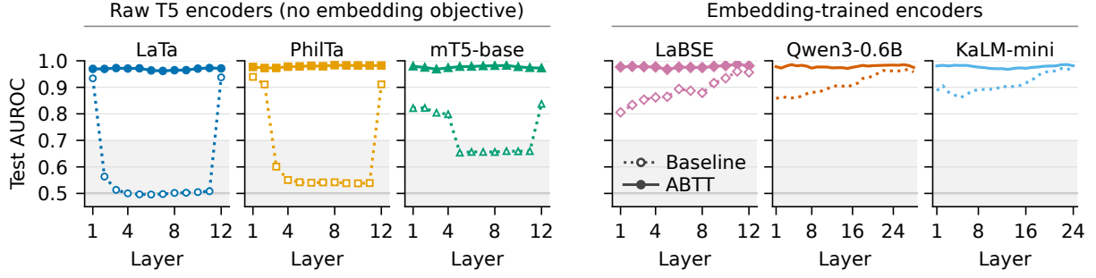
Figure 1: Test ranking AUROC at every layer of the six panel models. Dotted, open markers: baseline (mean-pooled hidden states). Solid, filled: ABTT (remove the training mean and the top D \leq 10 principal components), fit on training embeddings only. Gray band: AUROC below 0.70, the collapsed range; gray line: chance. The three raw T5 encoders collapse at mid-depth; after ABTT every layer scores 0.962 to 0.987.
