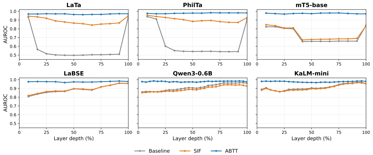
Figure 2: Task A AUROC against normalized layer depth for all six models. The three T5 encoders in the top row lose almost all pairwise separation in their middle layers, with LaTa reaching chance. The three sentence-embedding models in the bottom row improve close to monotonically with depth and never dip below 0.80. ABTT holds every model near its ceiling at every depth, so the repair does not depend on the collapse being present.
