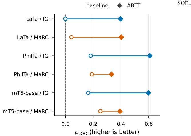
Figure 4: \rho_{\text{LOO}} foreground view for the main candidate-attribution result. Each line connects the baseline and ABTT variants for one model-method cell at the predeclared operational attribution layer. ABTT improves the leave-one-out rank-correlation signal in all six cells; Table 5 shows the ERASER-style disagreements which qualify this narrower faithfulness claim.
