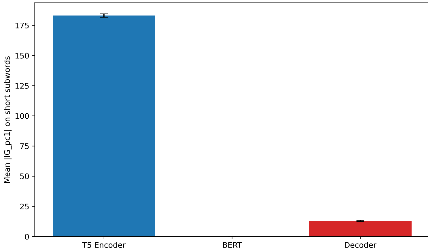
PC1 Loading of Short Subwords by Architecture
